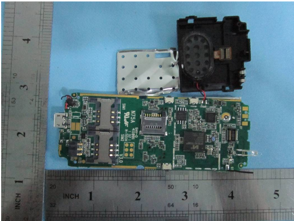
Mainboard Without Shielding - Bottom View
