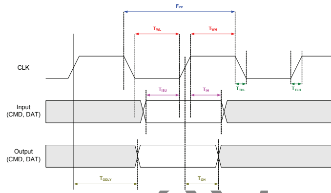
Figure 4-2. SDIO 2.0 Timing
