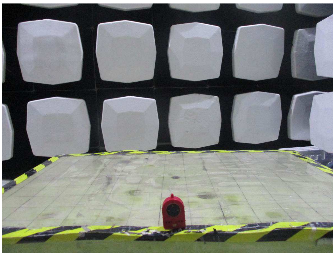
Up to 1GHz (The EUT placed at the center of the turntable)
