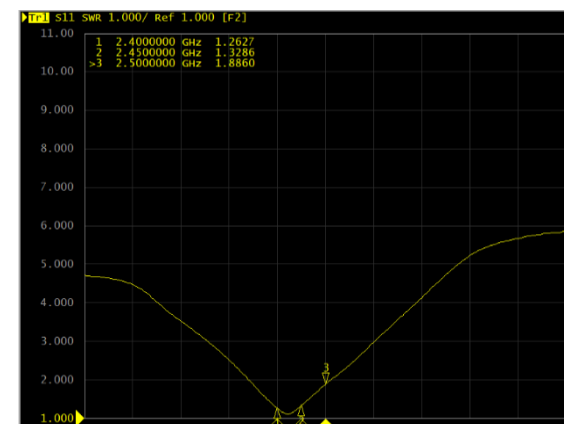
SWR
