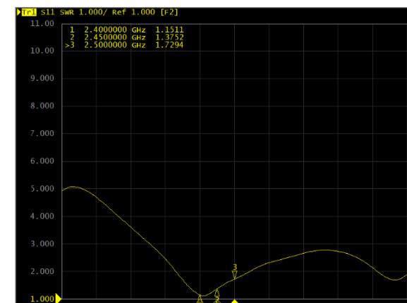
SWR
