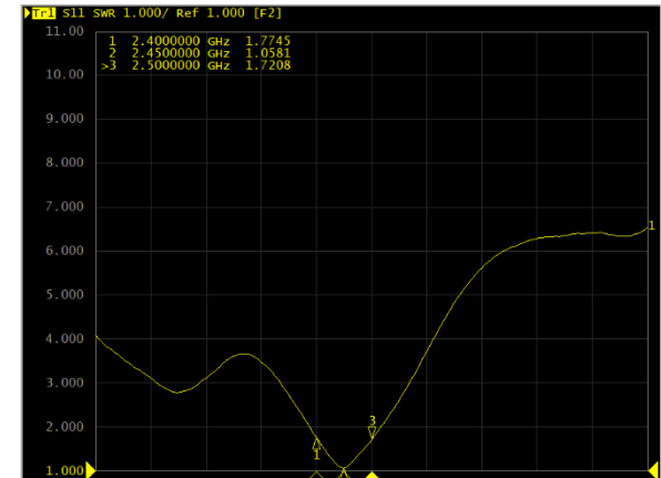
SWR
