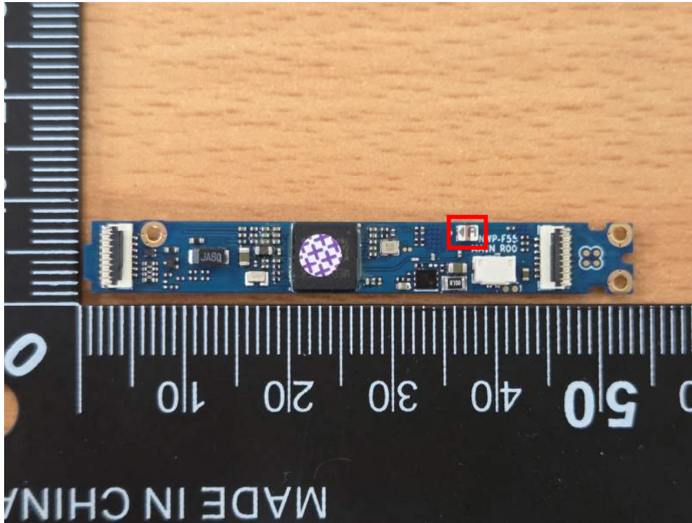
2402-2480MHz Antenna
