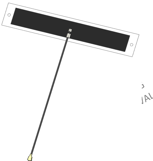
Molex 206764 868/915MHz Dipole Flexible Antenna 3D View
