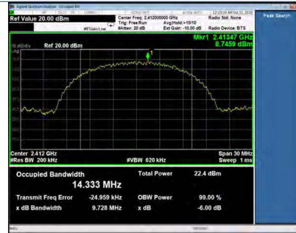
99% Bandwidth, Channel 1, 802.11b, 11Mbps
