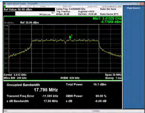
99% Bandwidth, Channel 1, 802.11n, MCS7
