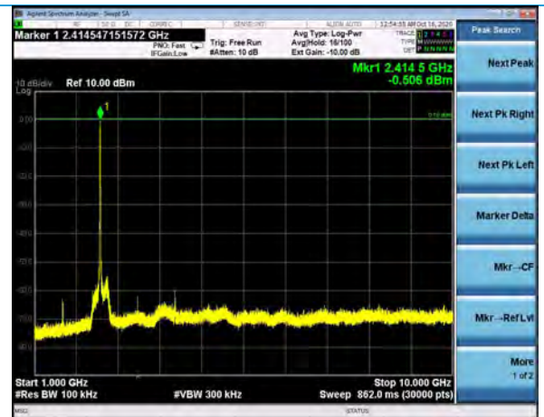
1-10 GHz, Channel 1, 802.11n, MCS0
