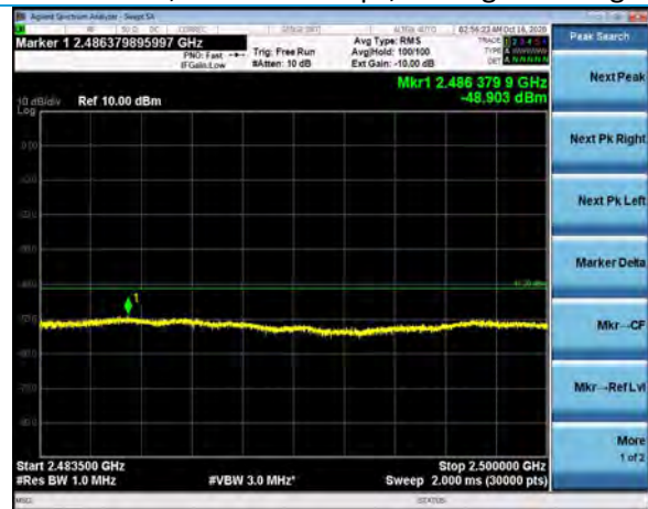
2.4835-2.5 GHz, Terminated Method, 1 MHz RBW Channel 11, 802.11b 1Mbps, Average Reading
