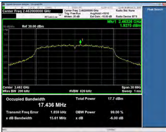
99% Bandwidth, Channel 11, 802.11n, MCS0
