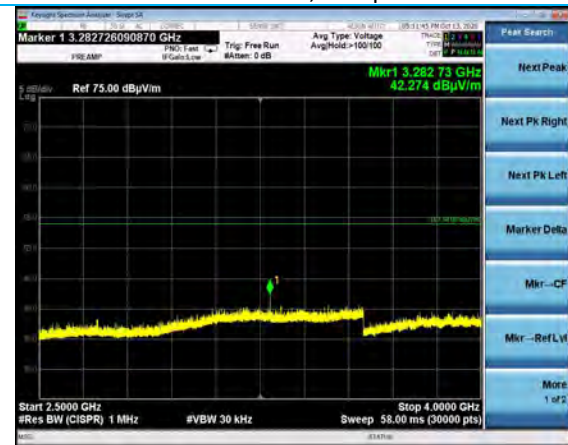
2500-4000 MHz, Vertical Antenna, Vertical EUT Channel 11
