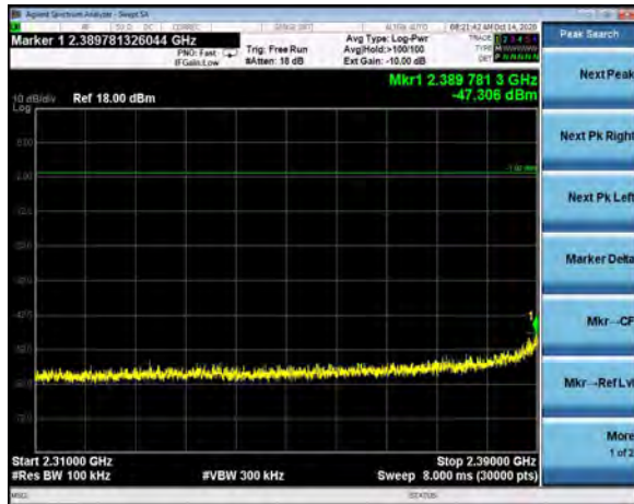
2310-2390 MHz, Channel 1, 802.11g, 54Mbps
