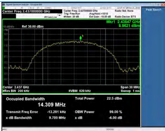
99% Bandwidth, Channel 6, 802.11b, 11Mbps
