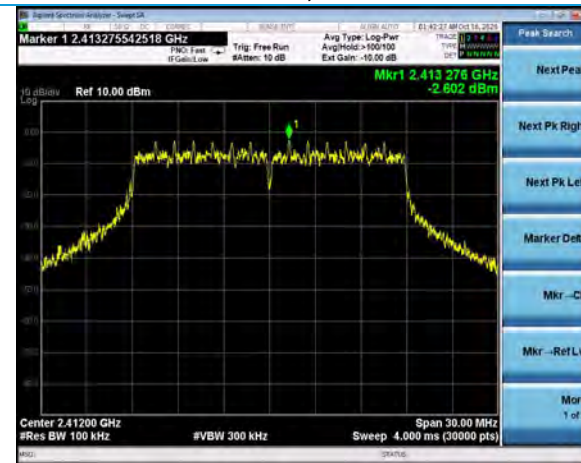
Reference Plot, 802.11n, MCS7 Channel 1, -2.6 dBm
