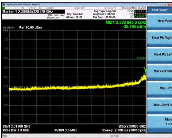
2.31-2.39 GHz, Terminated Method, 1 MHz RBW Channel 1, 802.11n MCS7, Peak Reading
