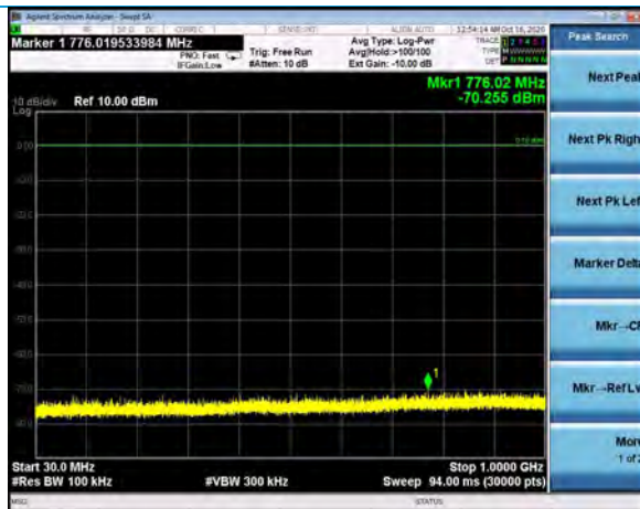
30-1000 MHz, Channel 1, 802.11n, MCS0
