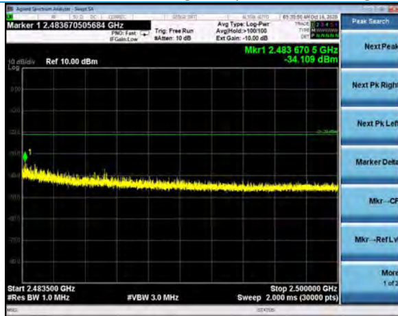
2.4835-2.5 GHz, Terminated Method, 1 MHz RBW Channel 11, 802.11g 6Mbps, Peak Reading
