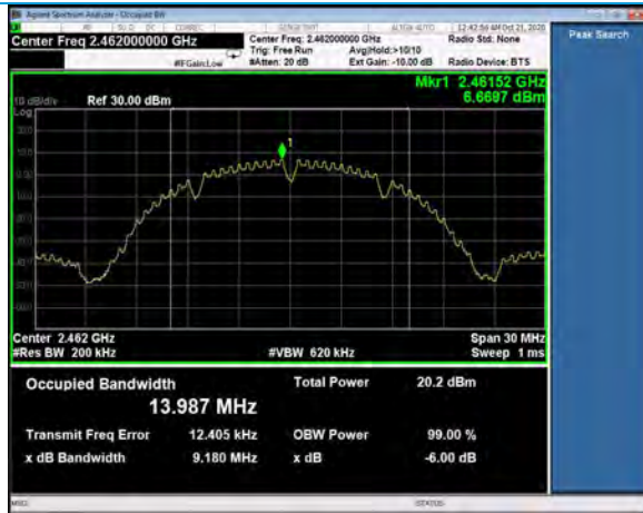
99% Bandwidth, Channel 11, 802.11b, 1Mbps
