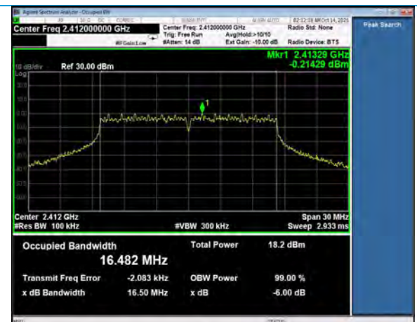
6 dB Bandwidth, Channel 1, 802.11g, 54Mbps
