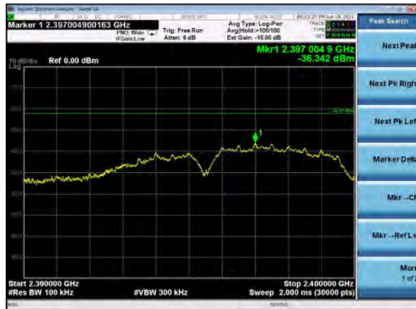
2390-2400 MHz, Channel 1, 802.11b, 1 Mbps
