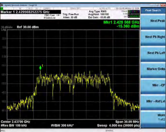
PSD, Channel 6, 802.11g, 54Mbps
