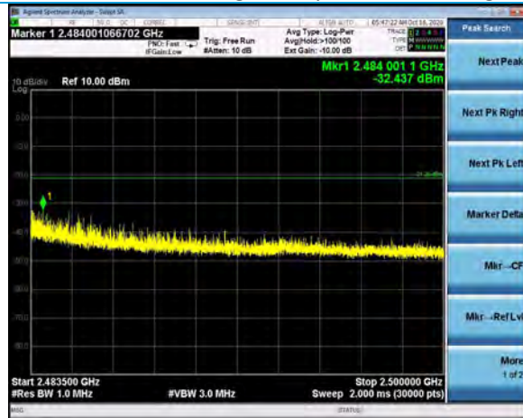
2.4835-2.5 GHz, Terminated Method, 1 MHz RBW Channel 11, 802.11g 54Mbps, Peak Reading
