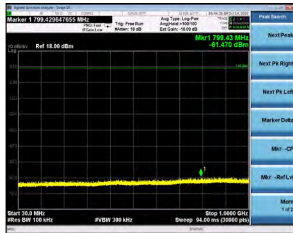
30-1000 MHz, Channel 1, 802.11b, 1Mbps
