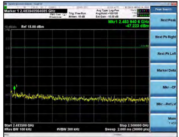
2483.5-2500 MHz, Channel 1, 802.11g, 54Mbps
