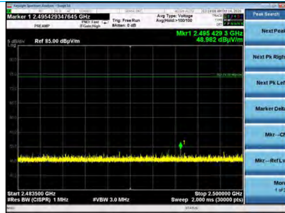
2483.5-2500 MHz, Horizontal Antenna, Flat EUT Channel 11, 1Mbps
