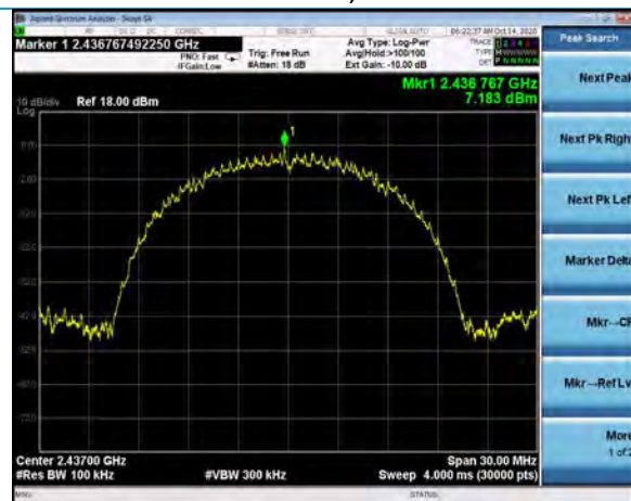
Reference Plot, 802.11b, 11Mbps Channel 6, 7.2 dBm
