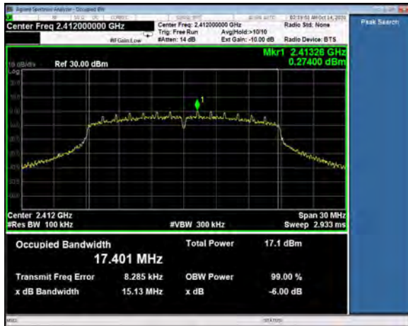
6 dB Bandwidth, Channel 1, 802.11n, MCS0
