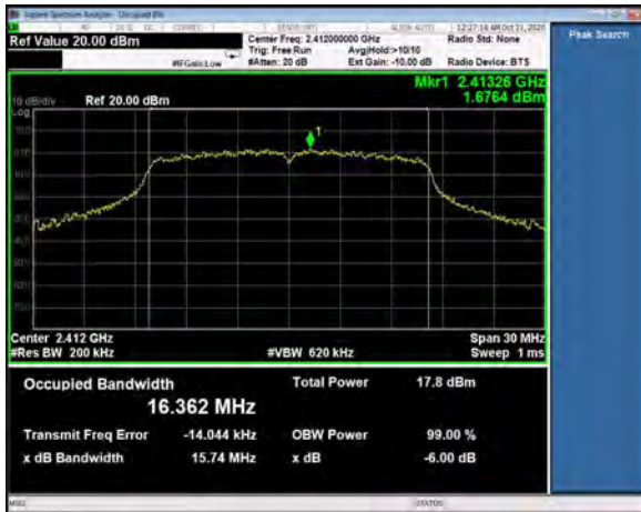
99% Bandwidth, Channel 1, 802.11g, 6Mbps
