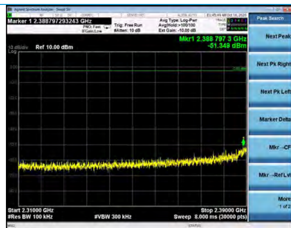
2310-2390 MHz, Channel 1, 802.11n, MCS7
