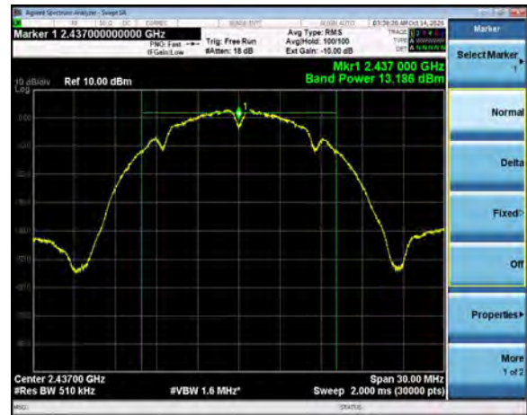
Output Power, Channel 6, 802.11b, 1Mbps
