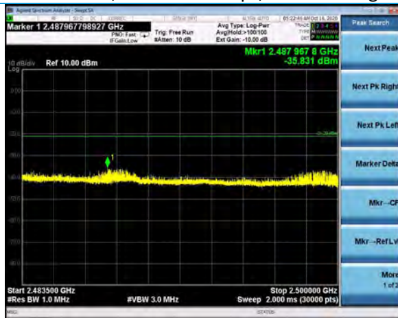
2.4835-2.5 GHz, Terminated Method, 1 MHz RBW Channel 11, 802.11b 11Mbps, Peak Reading
