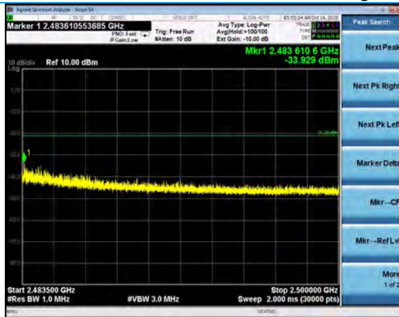
2.4835-2.5 GHz, Terminated Method, 1 MHz RBW Channel 11, 802.11n MCS0, Peak Reading
