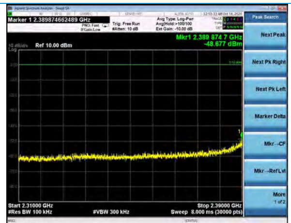
2310-2390 MHz, Channel 1, 802.11n, MCS0
