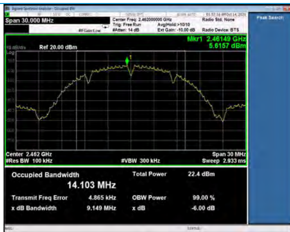
6 dB Bandwidth, Channel 11, 802.11b, 1Mbps
