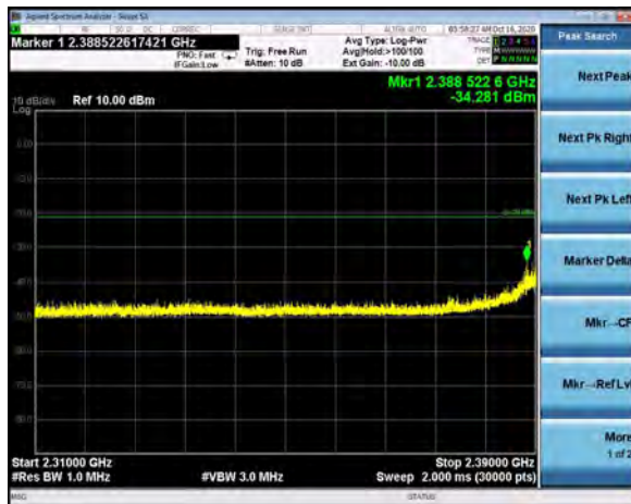
2.31-2.39 GHz, Terminated Method, 1 MHz RBW Channel 1, 802.11n MCS0, Peak Reading
