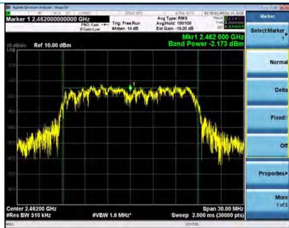
Output Power, Channel 11, 802.11n, MCS7
