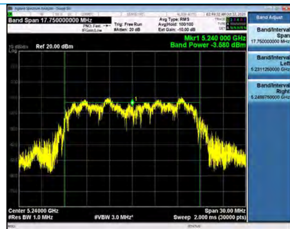
Output Power, Channel 48, 802.11n, MCS7
