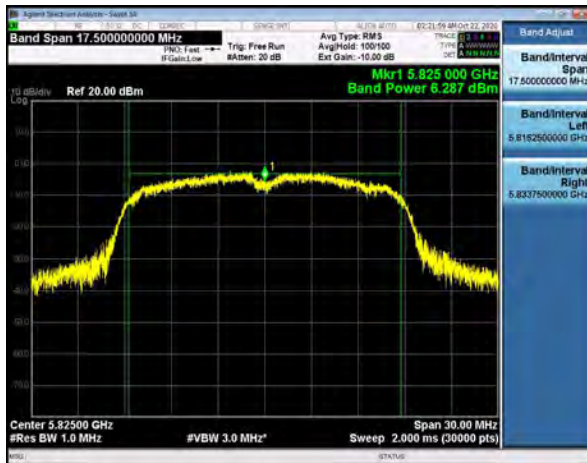
Output Power, Channel 165, 802.11n, MCS0
