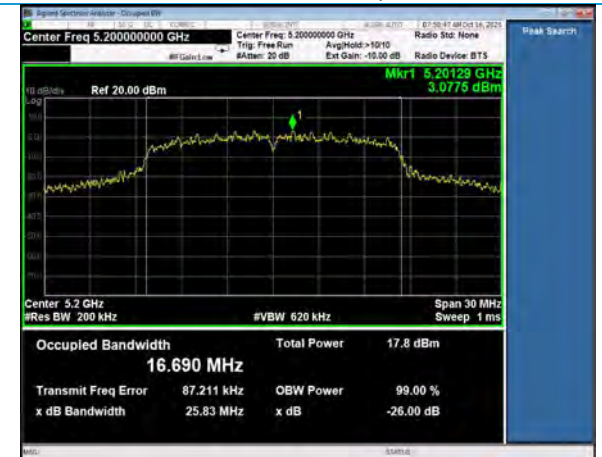
99% Occupied Bandwidth, Channel 40 802.11a, 6Mbps
