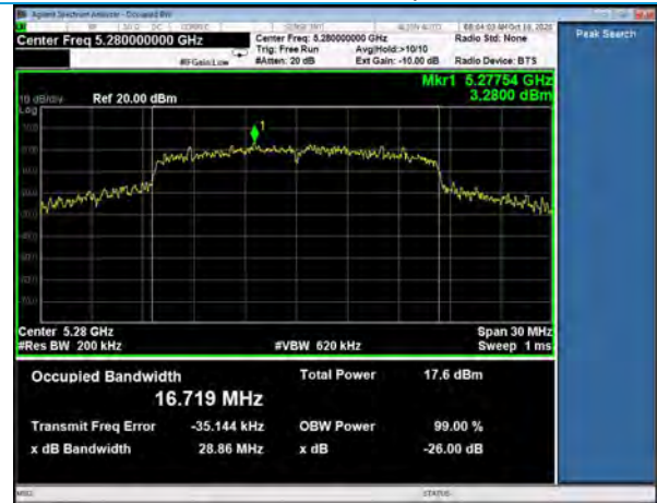
99% Occupied Bandwidth, Channel 56 802.11a, 6Mbps
