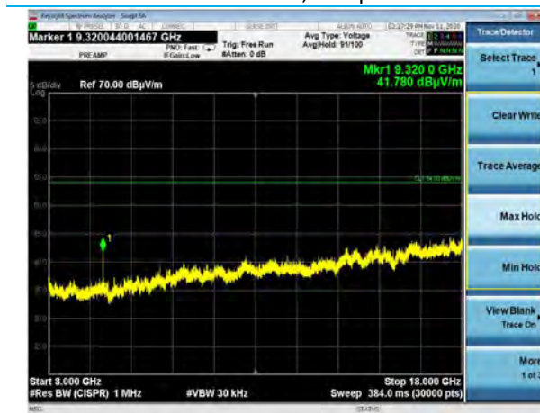
8-18 GHz, Horizontal Antenna, Flat EUT Channel 165, 6Mbps
