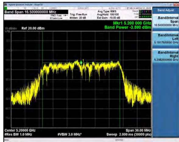
Output Power, Channel 40, 802.11a, 54Mbps
