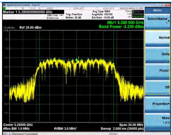
Output Power, Channel 56, 802.11a, 54Mbps
