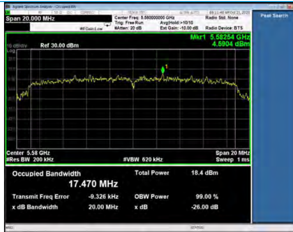
26 dB Emission Bandwidth, Channel 116 802.11n, MCS0
