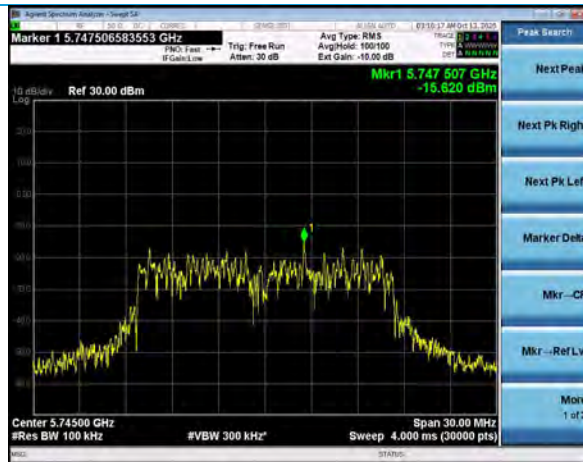
PSD, Channel 149, 802.11a, 54Mbps
