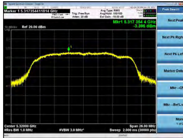
PSD, Channel 64, 802.11n, MCS0
