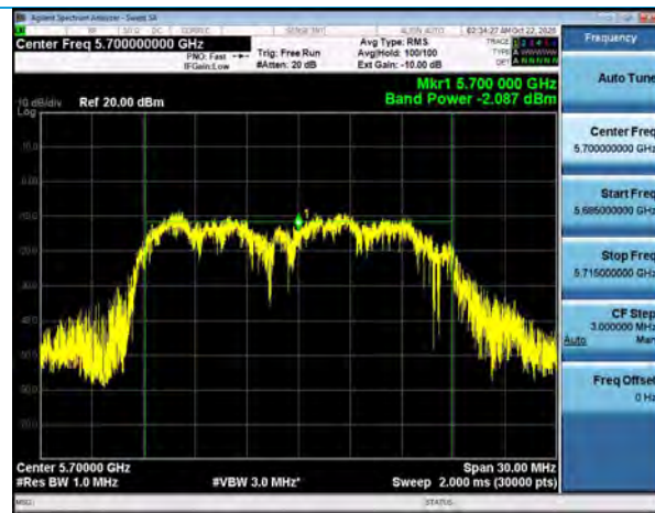
Output Power, Channel 140, 802.11n, MCS7
