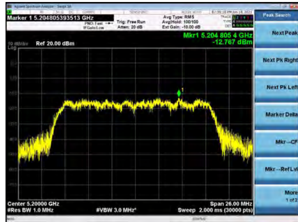
PSD, Channel 40, 802.11a, 54Mbps
