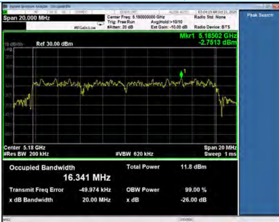
99% Occupied Bandwidth, Channel 36 802.11a, 6Mbps
