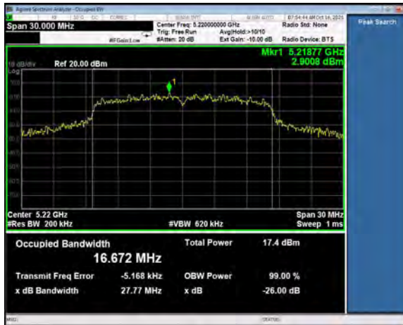
99% Occupied Bandwidth, Channel 44 802.11a, 6Mbps
