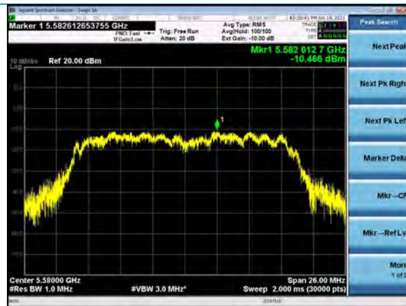
PSD, Channel 116, 802.11n, MCS7
