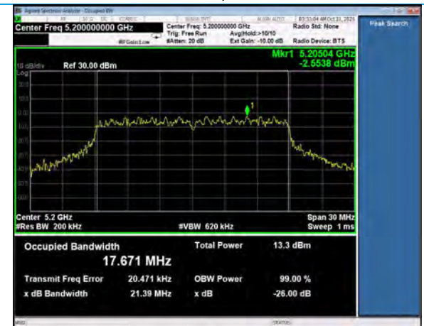
99% Occupied Bandwidth, Channel 40 802.11n, MCS7
