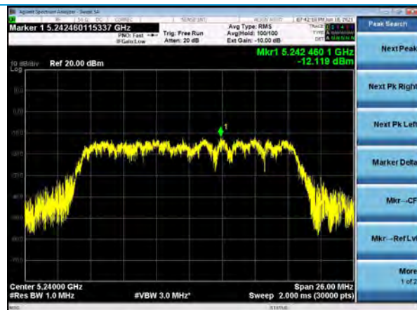
PSD, Channel 48, 802.11a, 54Mbps
