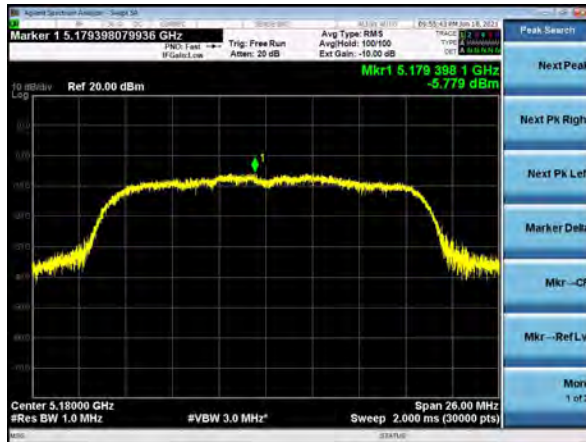
PSD, Channel 36, 802.11n, MCS0
