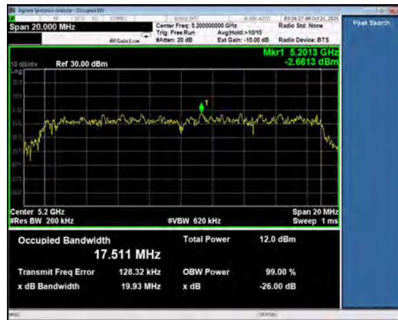
26 dB Emission Bandwidth, Channel 40 802.11n, MCS0
