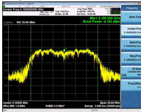
Output Power, Channel 36, 802.11n, MCS7
