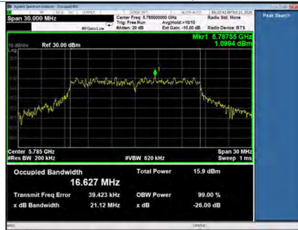
99% Occupied Bandwidth, Channel 157 802.11a, 54Mbps
