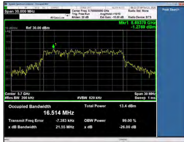
99% Occupied Bandwidth, Channel 140 802.11a, 54Mbps
