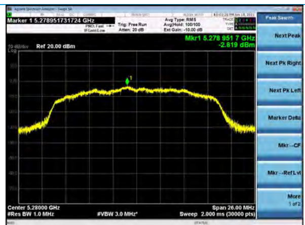
PSD, Channel 56, 802.11n, MCS0
