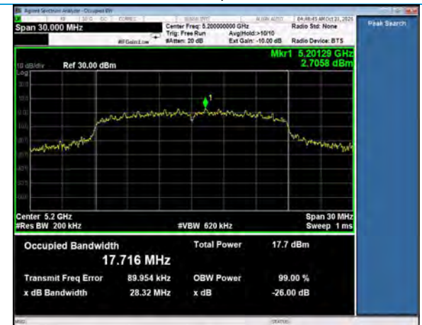
99% Occupied Bandwidth, Channel 40 802.11n, MCS0
