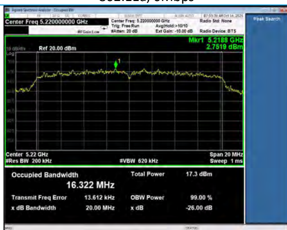
26 dB Emission Bandwidth, Channel 44 802.11a, 6Mbps
