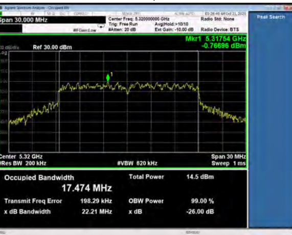
99% Occupied Bandwidth, Channel 64 802.11n, MCS7
