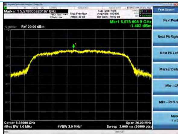
PSD, Channel 116, 802.11n, MCS0
