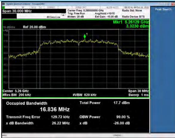
99% Occupied Bandwidth, Channel 52 802.11a, 6Mbps
