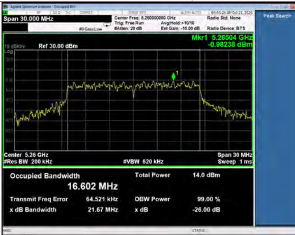
99% Occupied Bandwidth, Channel 52 802.11a, 54Mbps
