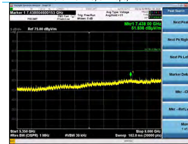
5350-8000 MHz, Horizontal Antenna, Flat EUT Channel 48, 6Mbps
