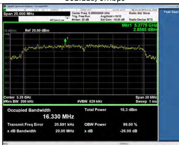
26 dB Emission Bandwidth, Channel 56 802.11a, 6Mbps
