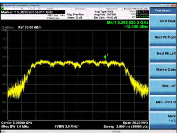
PSD, Channel 52, 802.11n, MCS7
