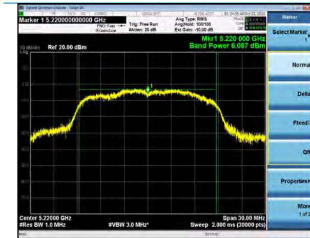
Output Power, Channel 44, 802.11n, MCS0
