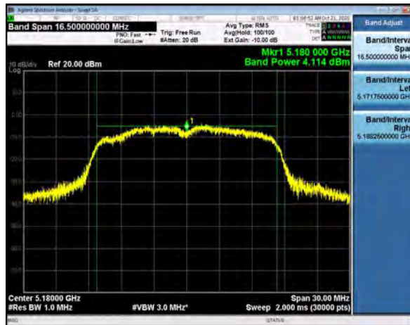
Output Power, Channel 36, 802.11a, 6Mbps
