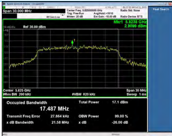
99% Occupied Bandwidth, Channel 165 802.11n, MCS0
