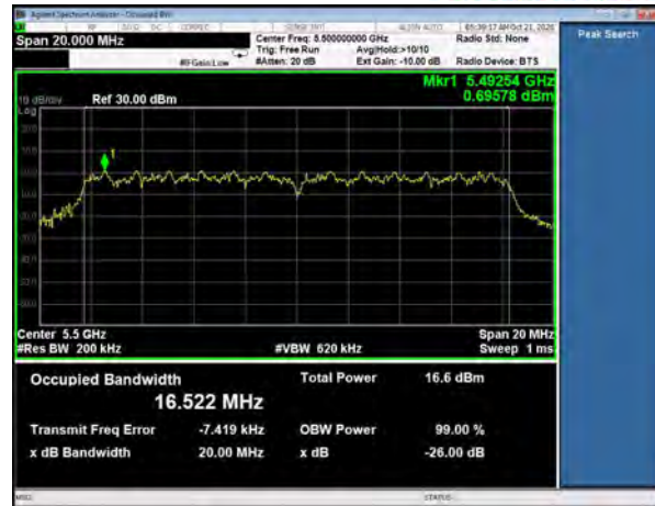
26 dB Emission Bandwidth, Channel 100 802.11a, 54Mbps
