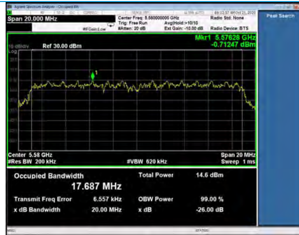
26 dB Emission Bandwidth, Channel 116 802.11n, MCS7
