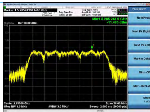
PSD, Channel 56, 802.11a, 54Mbps
