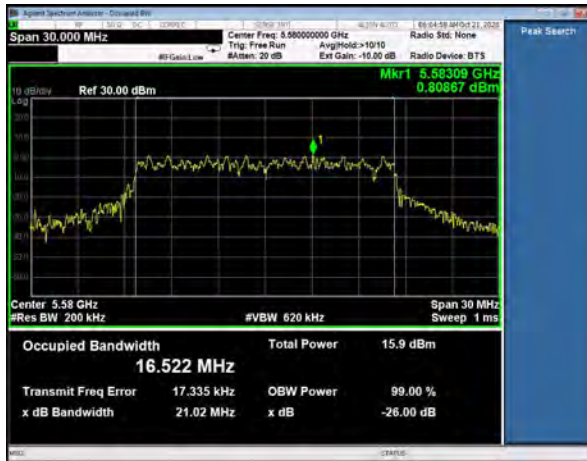
99% Occupied Bandwidth, Channel 116 802.11a, 54Mbps
