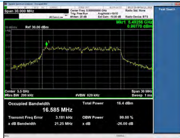
99% Occupied Bandwidth, Channel 100 802.11a, 54Mbps
