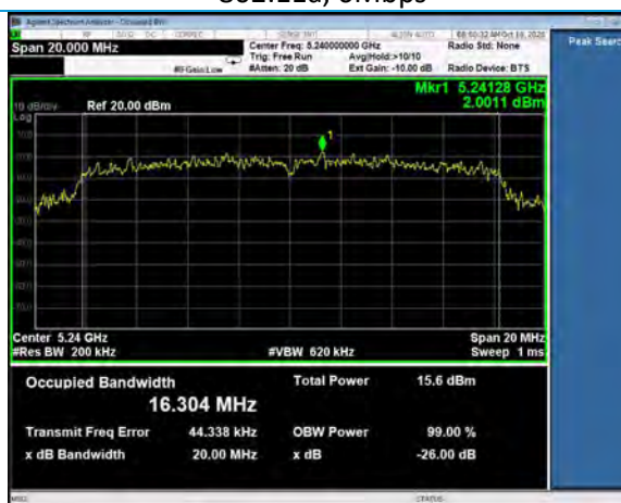
26 dB Emission Bandwidth, Channel 48 802.11a, 6Mbps
