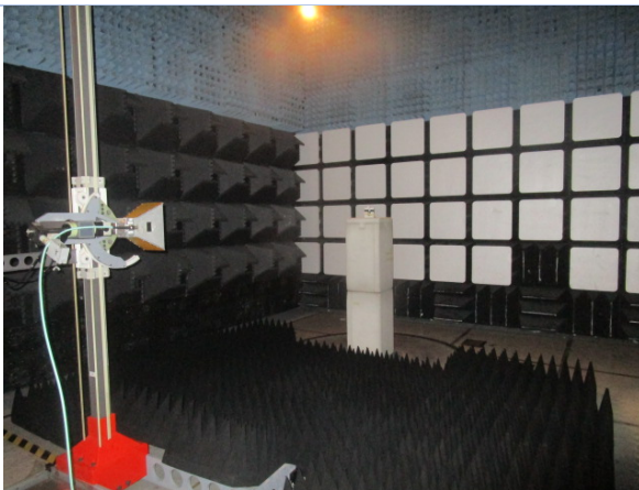
Chamber 3 Radiated Emissions Setup
