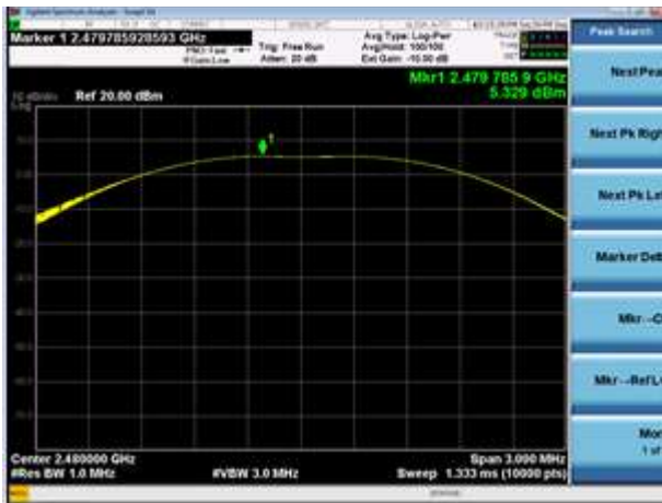
Worst Case Conducted Peak Output Power BLE, 2480 MHz
