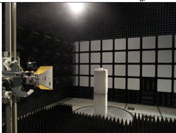
Radiated Emissions
