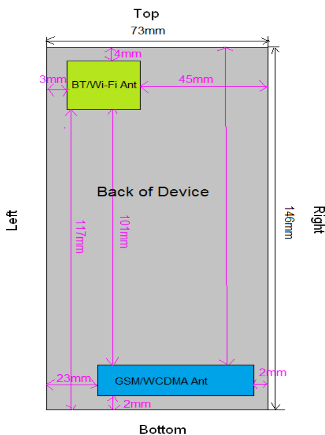
Mobile Hotspot Sides for SAR Testing
