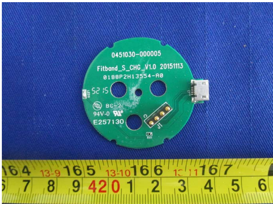
EUT – Charger Board Top View
