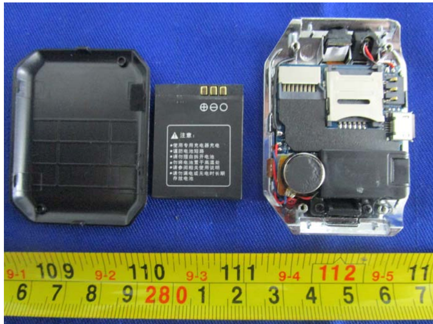
EUT – Cover Removed 1 View
