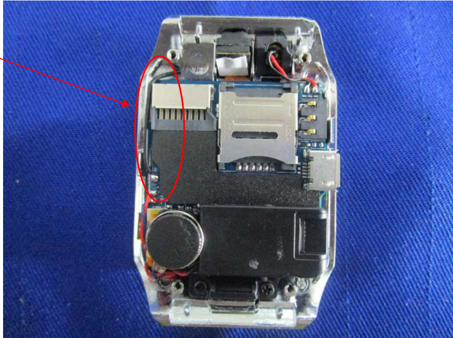
EUT – Cover Removed 2 View
