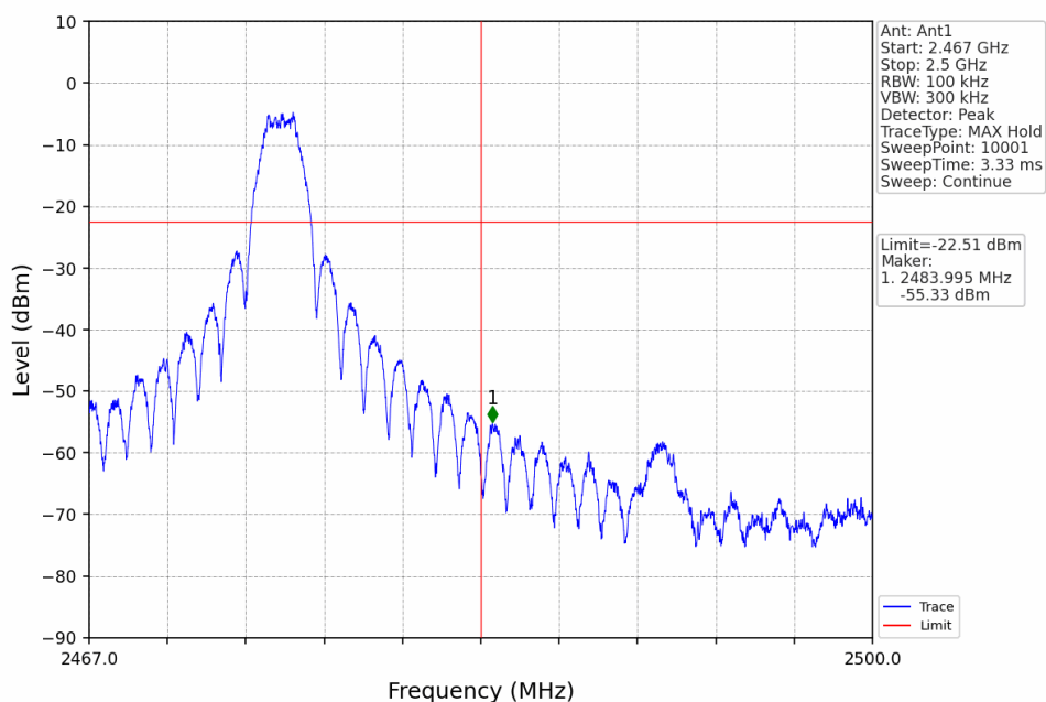
2.4g_HCH_2475MHz_Ant1_NTNV
