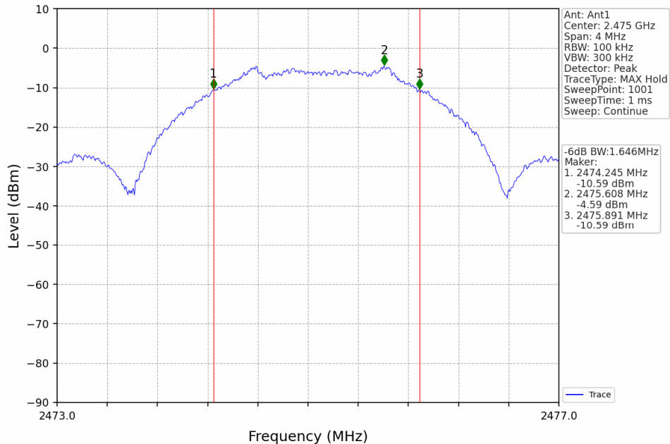
2.4g_HCH_2475MHz_Ant1_NTNV
