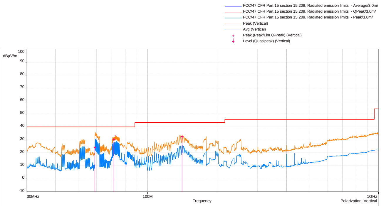
30MHz – 1 GHz_Vertical Polarization with user cycling Mode
