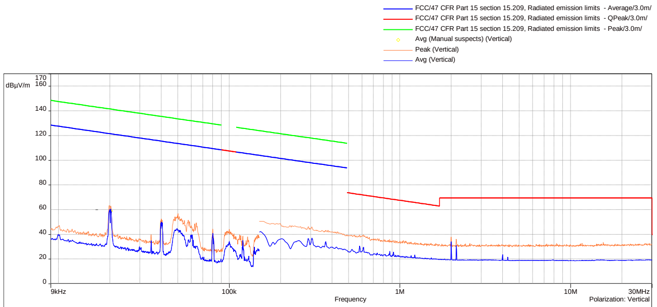
Parallel Polarization_9kHz to 30 MHz
