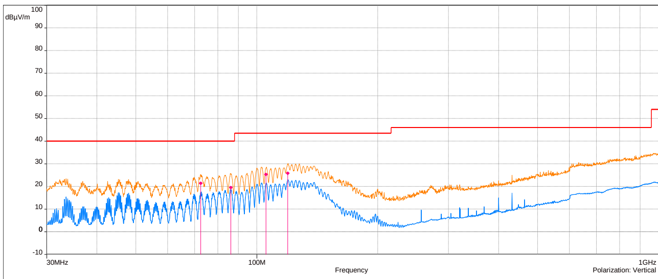
30 MHz – 1 GHz_Vertical Polarization
