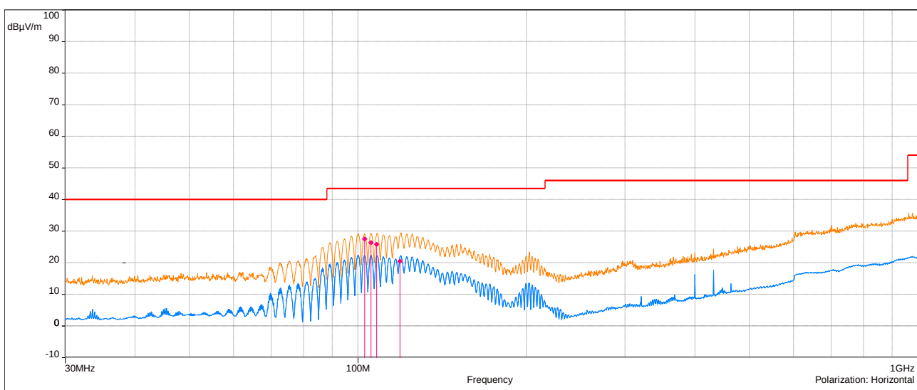
30 MHz – 1 GHz_Horizontal Polarization
