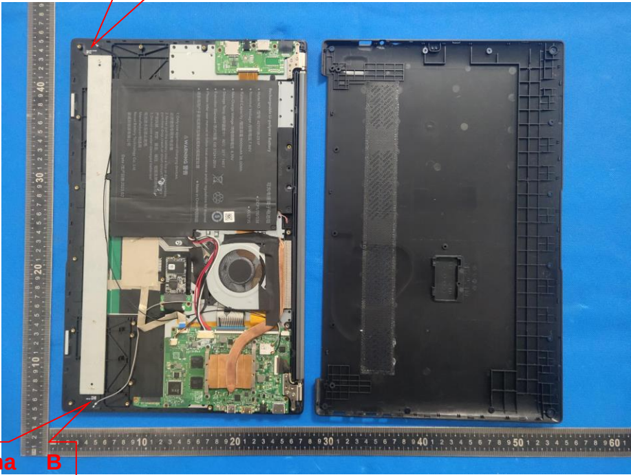
Internal Photos Antenna A BT/WIFI
