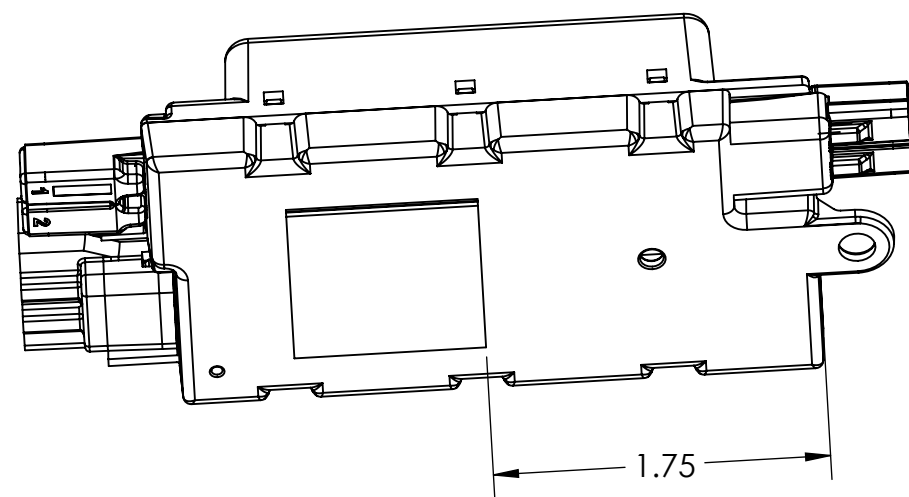
VIEW A-A SEE NOTE #4
