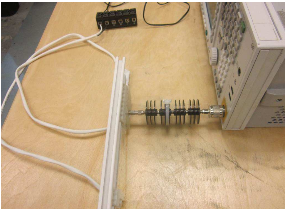
Conducted Testing at Antenna port (Closed up View)
