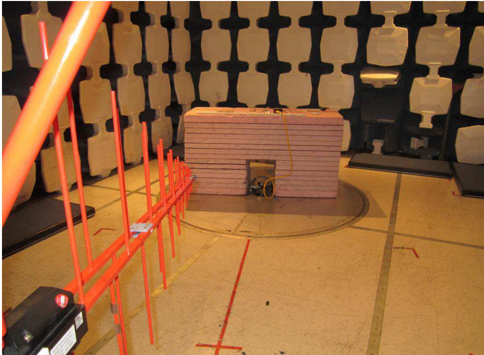
Radiated Emissions – Mid range
