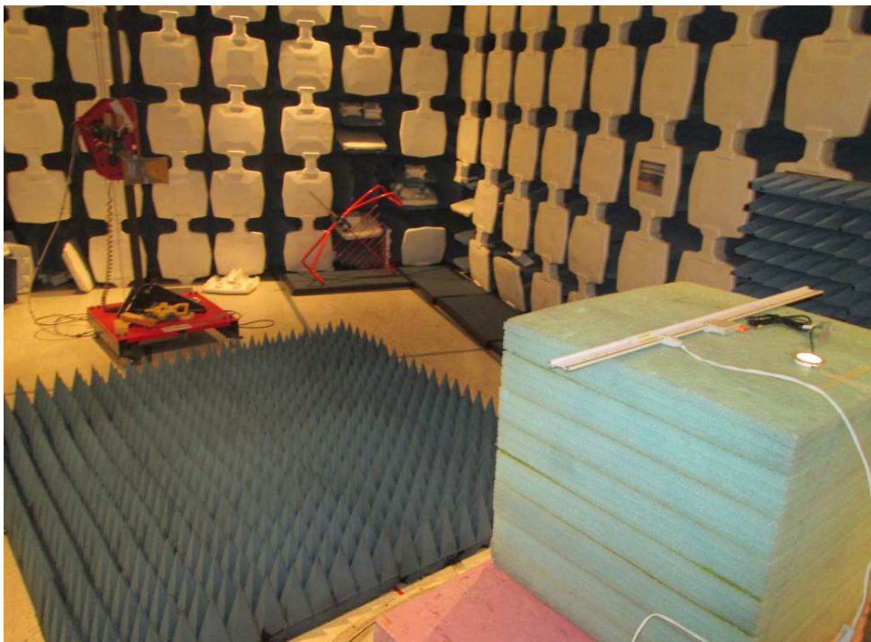
Radiated Emissions – 1 to 6 GHz
