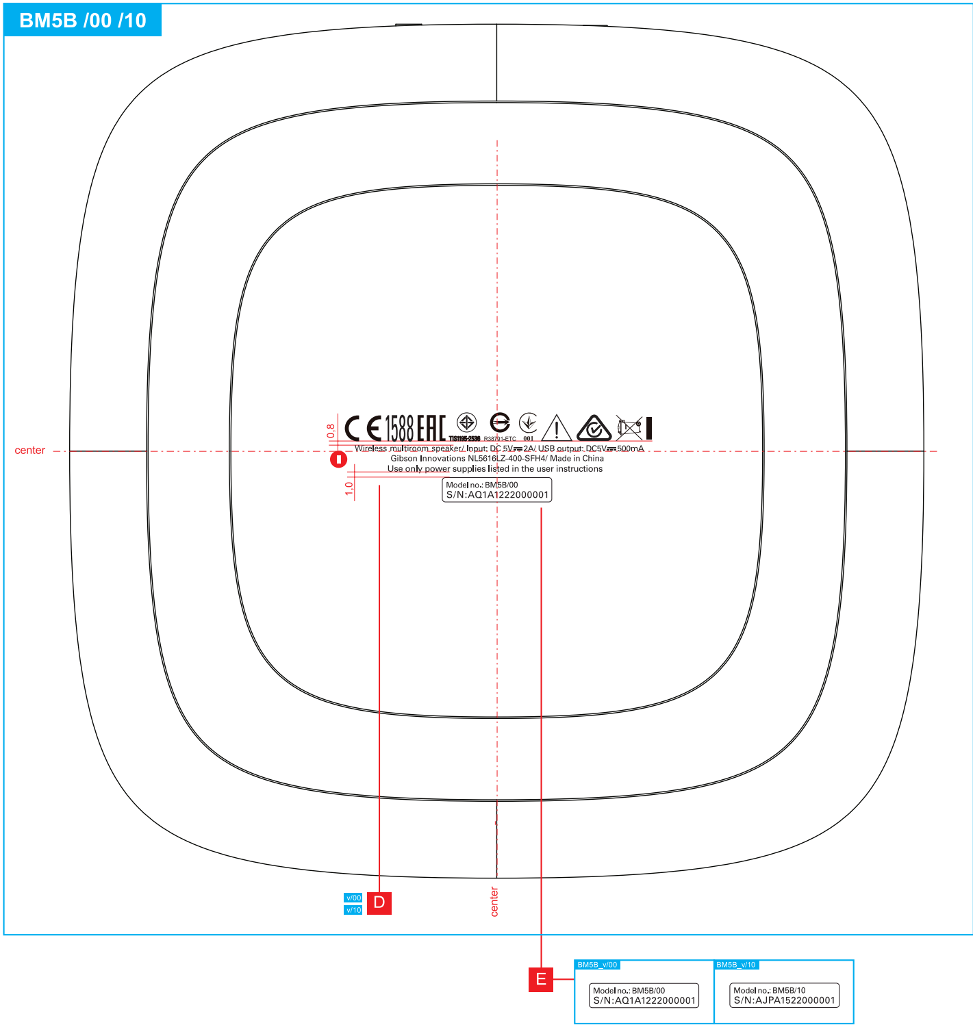
Bottom view
