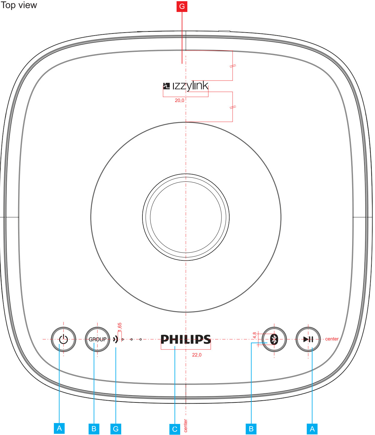
Top view
