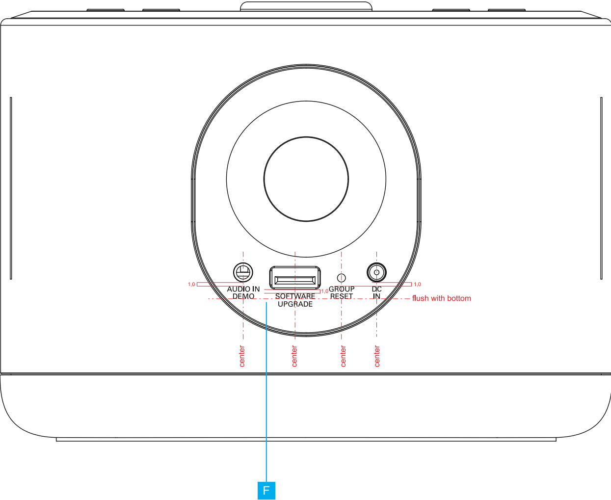
Front view
