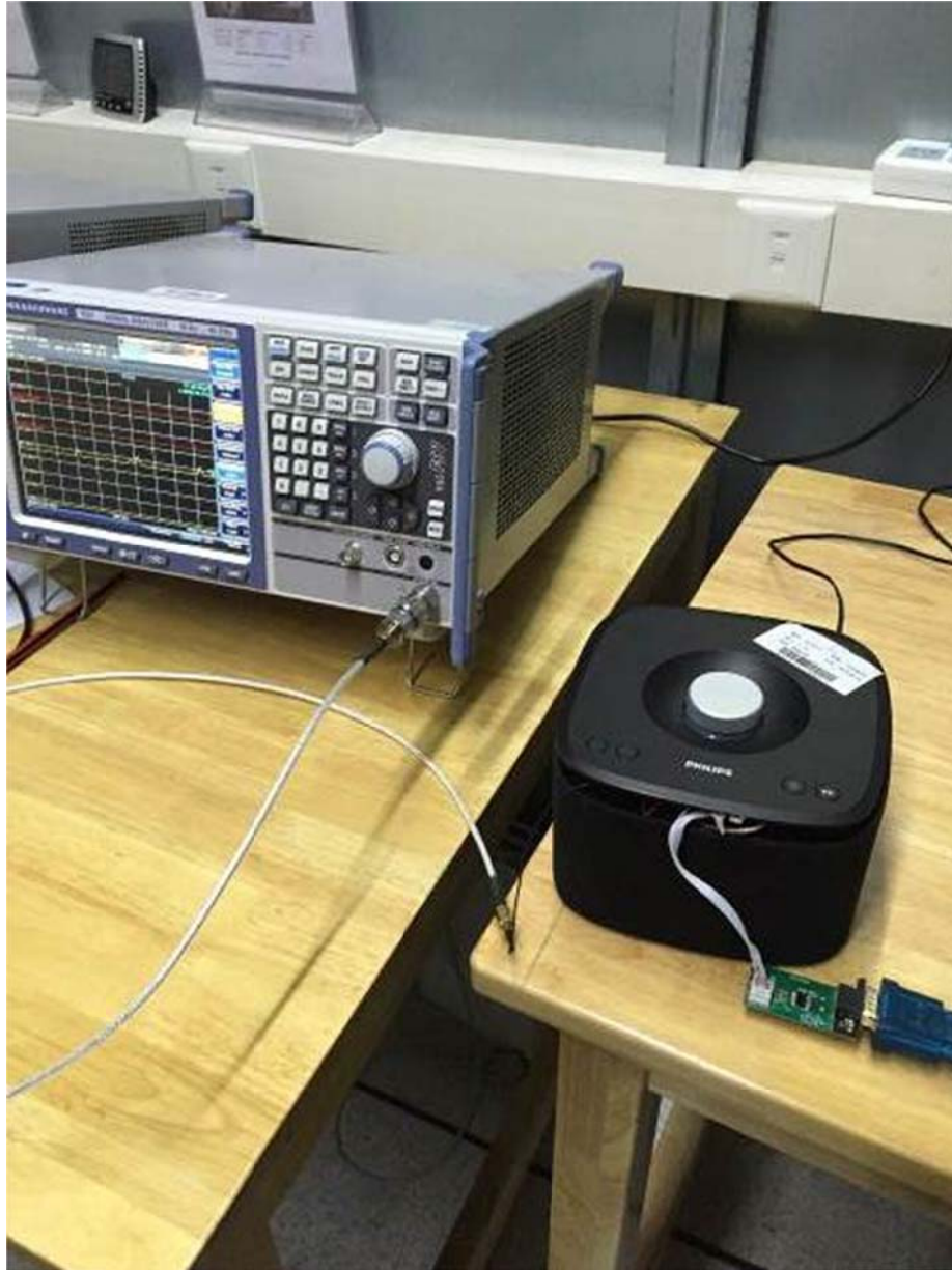
Figure 1 Conducted measurement Test setup for BT test
