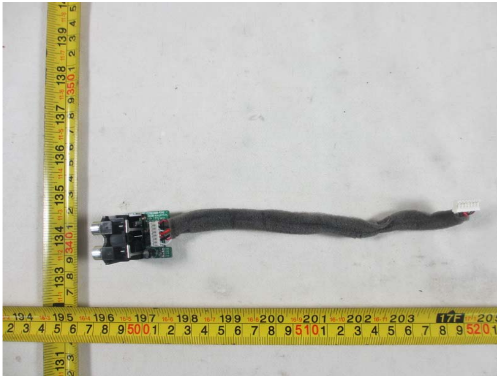
Accessory board
