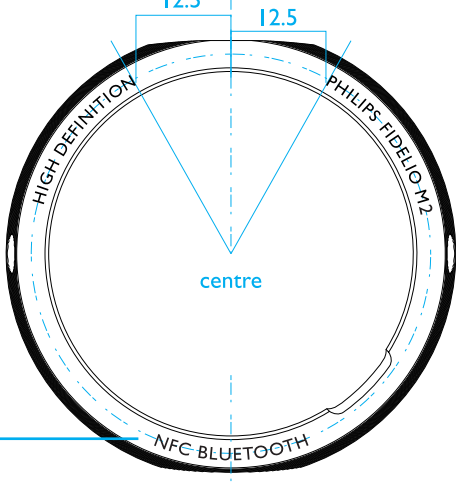
[08R] Ear shell RIGHT_ O-ring
