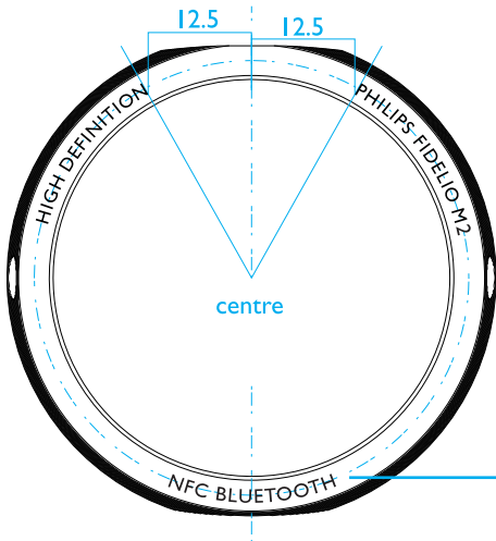
[08L] Ear shell LEFT_ O-ring
