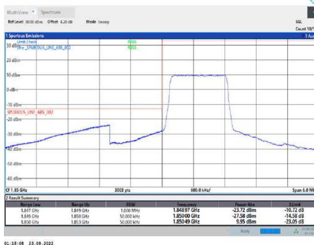
Band2-1.4MHz-QPSK-18607-6RB#0
