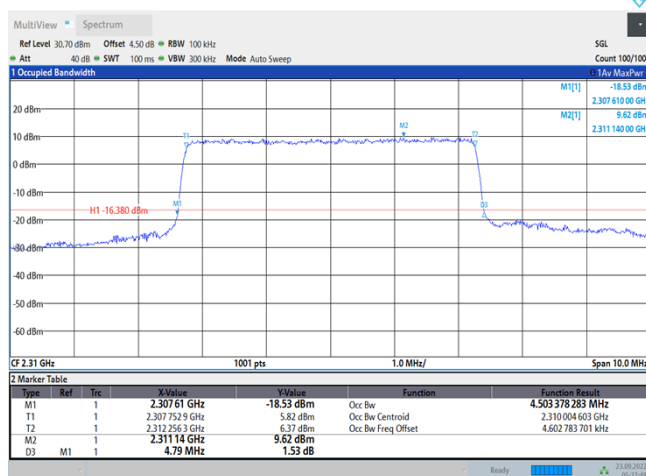
Band30-5MHz-QPSK-27710-25RB#0
