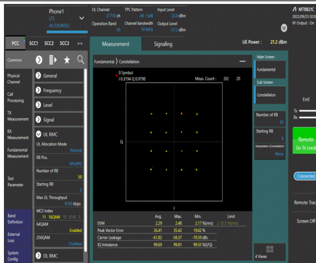
Band30-10MHz-16QAM-27710-50RB#0
