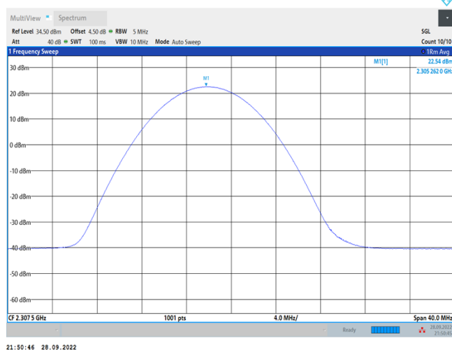
Band30-5MHz-QPSK-27685-1RB#24
