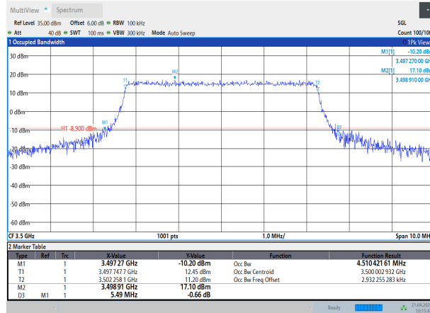
Band42-5MHz-QPSK-42590-25RB#0
