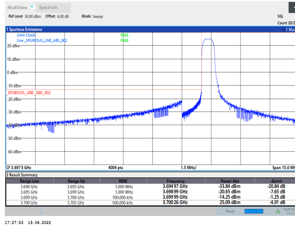
Band43-5MHz-QPSK-44615-25RB#0
