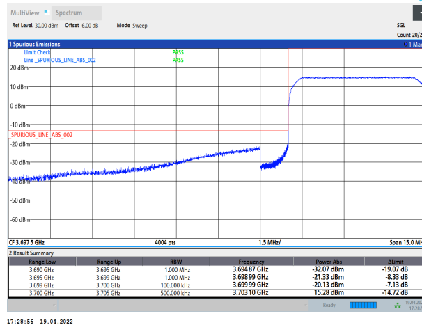
Band43-5MHz-QPSK-44615-25RB#0
