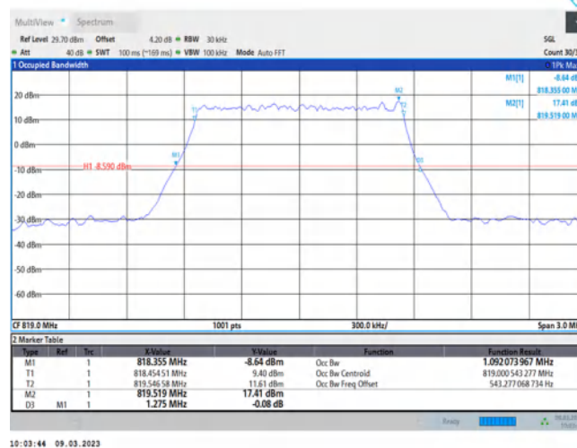
Band26-1.4MHz-QPSK-26740-6RB#0
