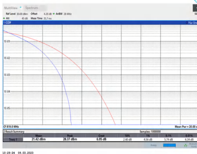
Band26-10MHz-16QAM-26740-50RB#0
