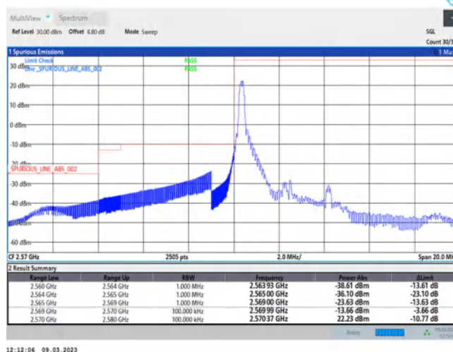
Band38-5MHz-QPSK-37775-25RB#0
