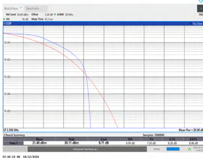
Band41-20MHz-QPSK-40620-100RB#0
