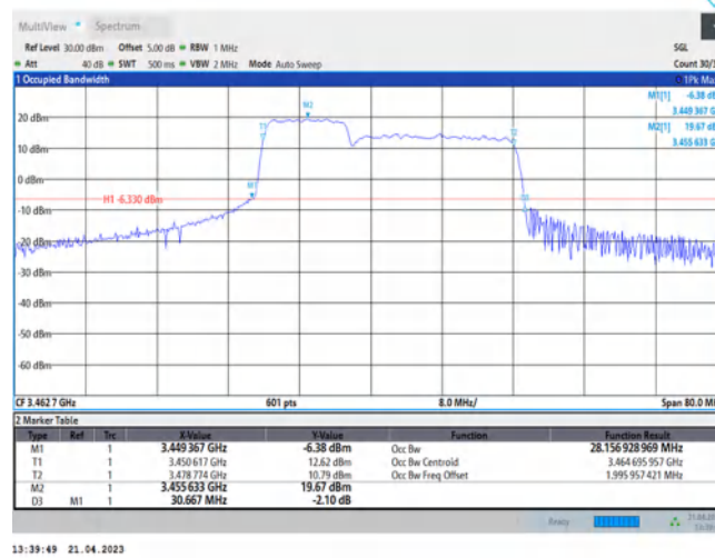
42-42-10MHz-20MHz-QPSK-QPSK-42496-42640-50RB#0-100RB#0
