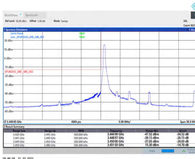
42-42-10MHz-20MHz-QPSK-QPSK-42145-42289-50RB#0-100RB#0
