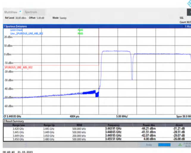
42-42-10MHz-20MHz-QPSK-QPSK-42145-42289-50RB#0-100RB#0
