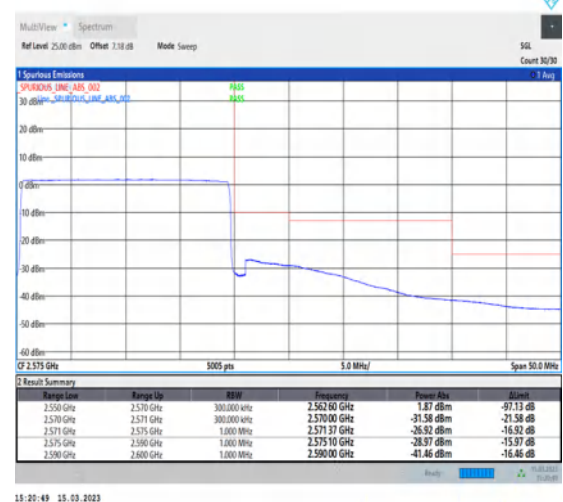
1-N7-PC3-15-20-H-6-CP-QPSK-Outer_Full-106@0-Ant1-1--PASS-see graph
