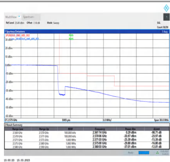
1-N7-PC3-15-10-H-6-CP-QPSK-Outer_Full-52@0-Ant1-1--PASS-see graph
