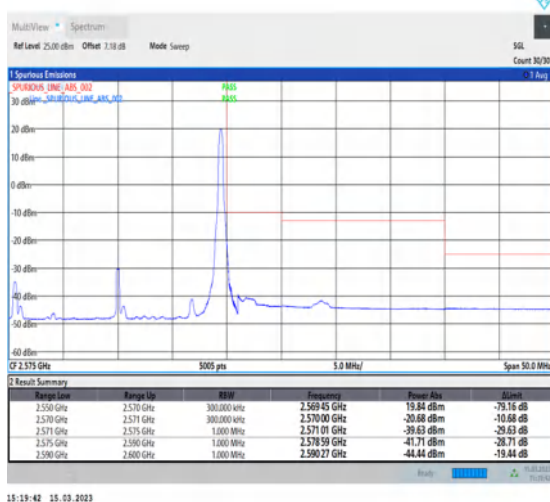
1-N7-PC3-15-20-H-5-CP-QPSK-Edge_1RB_Right-1@105-Ant1-1--PASS-see graph
