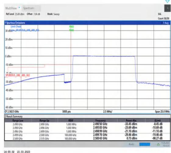
1-N7-PC3-15-10-L-6-CP-QPSK-Outer_Full-52@0-Ant1-1--PASS-see graph
