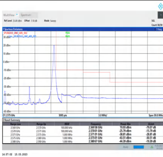
1-N7-PC3-15-10-H-2-DFT-PI2BPSK-Edge_1RB_Right-1@51-Ant1-1--PASS-see graph
