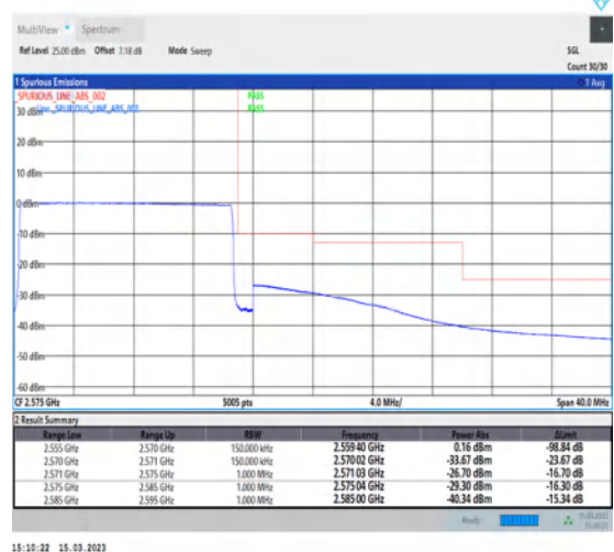
1-N7-PC3-15-15-H-6-CP-QPSK-Outer_Full-79@0-Ant1-1--PASS-see graph
