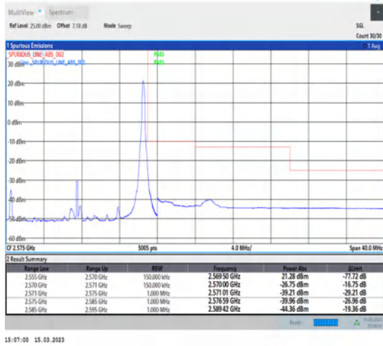
1-N7-PC3-15-15-H-2-DFT-PI2BPSK-Edge_1RB_Right-1@78-Ant1-1--PASS-see graph
