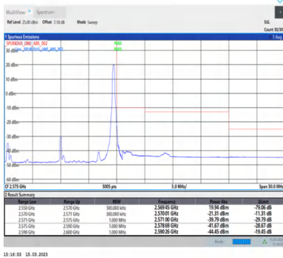
1-N7-PC3-15-20-H-2-DFT-PI2BPSK-Edge_1RB_Right-1@105-Ant1-1--PASS-see graph
