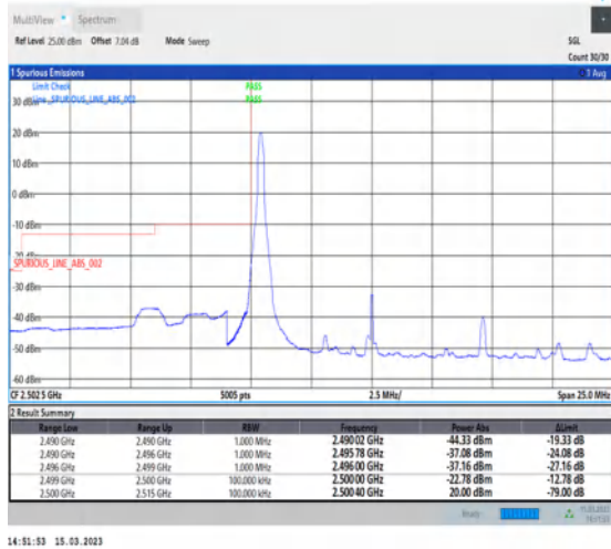
1-N7-PC3-15-10-L-1-DFT-PI2BPSK-Edge_1RB_Left-1@0-Ant1-1--PASS-see graph
