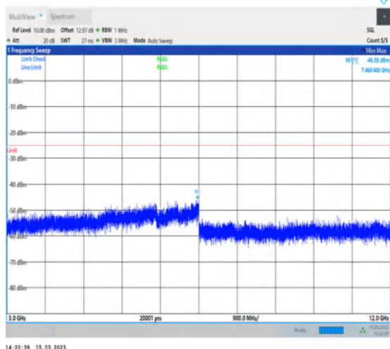
1-N7-PC3-15-20-M-1-DFT-PI2BPSK- Inner_1RB_Left-1@1-3000-12000-Ant1-7460.40-- 46.03--25-PASS
