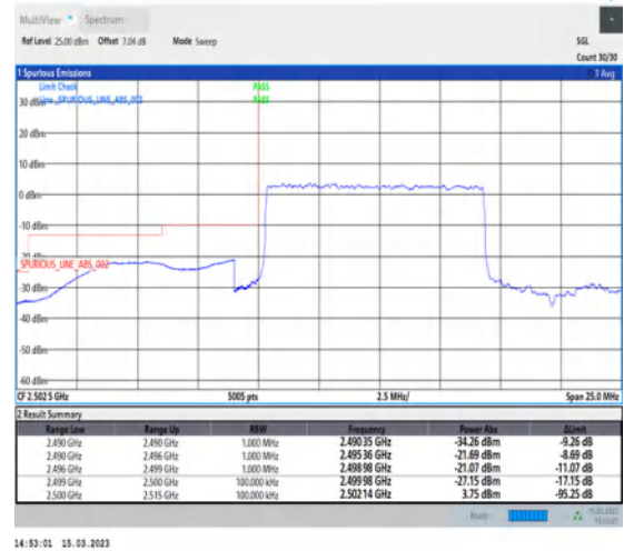
1-N7-PC3-15-10-L-3-DFT-PI2BPSK-Outer_Full-50@0-Ant1-1--PASS-see graph
