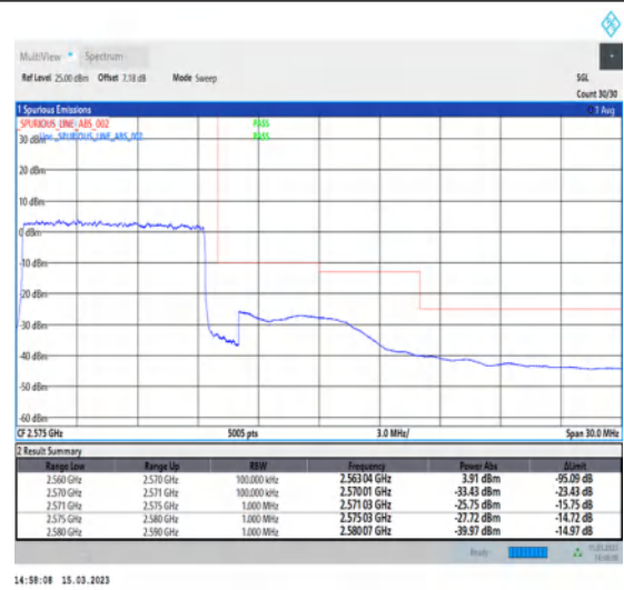
1-N7-PC3-15-10-H-3-DFT-PI2BPSK-Outer_Full-50@0-Ant1-1--PASS-see graph
