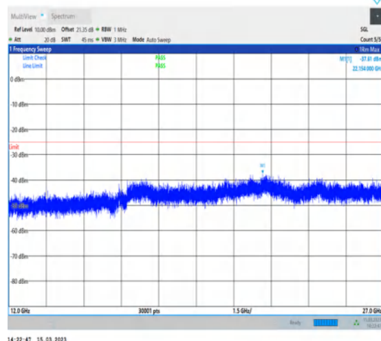
1-N7-PC3-15-20-M-1-DFT-PI2BPSK- Inner_1RB_Left-1@1-12000-27000-Ant1-22154.00-- 37.61--25-PASS
