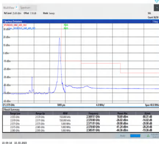
1-N7-PC3-15-15-H-5-CP-QPSK-Edge_1RB_Right-1@78-Ant1-1--PASS-see graph
