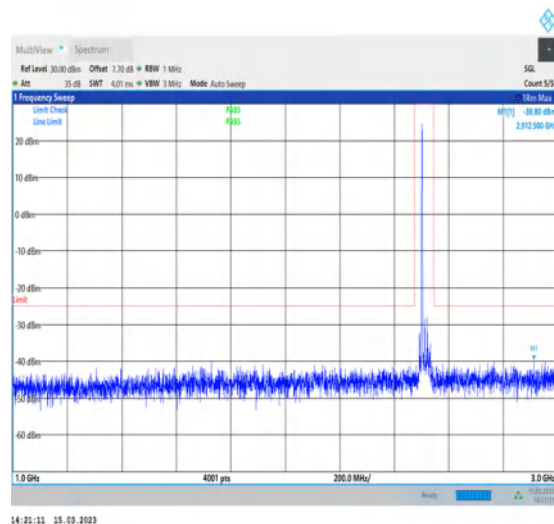
1-N7-PC3-15-20-L-1-DFT-PI2BPSK-Inner_1RB_Left- 1@1-1000-3000-Ant1-2912.50--39.80--25-PASS
