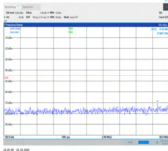
1-N7-PC3-15-20-L-1-DFT-PI2BPSK-Inner_1RB_Left- 1@1-0.15-30-Ant1-27.88--72.28--45-PASS
