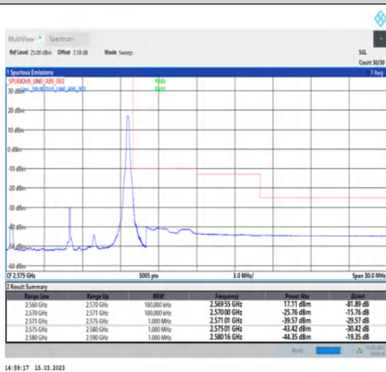
1-N7-PC3-15-10-H-5-CP-QPSK-Edge_1RB_Right-1@51-Ant1-1--PASS-see graph
