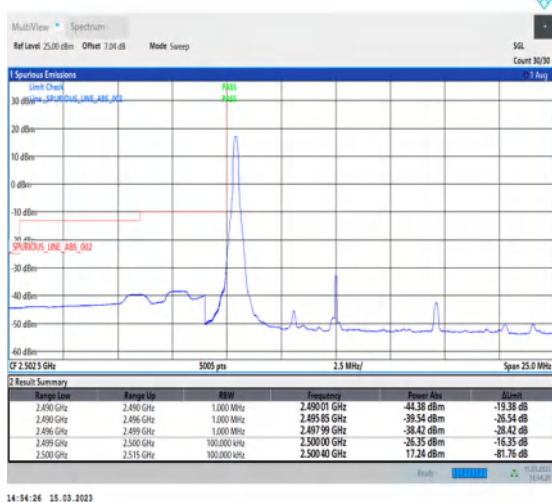
1-N7-PC3-15-10-L-4-CP-QPSK-Edge_1RB_Left-1@0-Ant1-1--PASS-see graph
