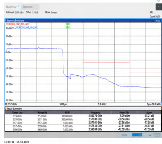
1-N7-PC3-15-20-H-3-DFT-PI2BPSK-Outer_Full-100@0-Ant1-1--PASS-see graph
