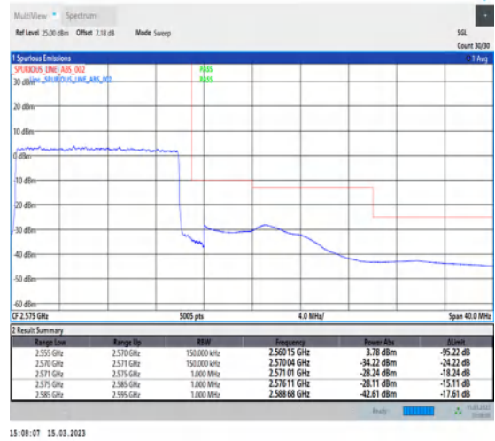
1-N7-PC3-15-15-H-3-DFT-PI2BPSK-Outer_Full-75@0-Ant1-1--PASS-see graph
