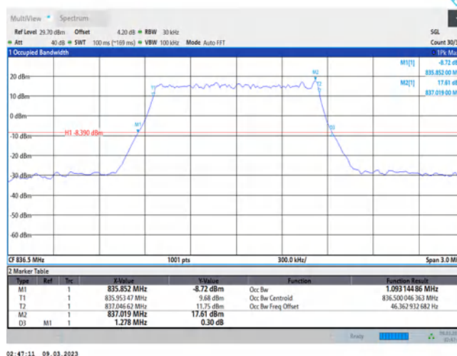
Band5-1.4MHz-QPSK-20525-6RB#0
