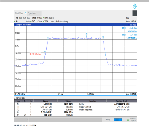
Band70-15MHz-256QAM-133047-75RB#0-PASS
