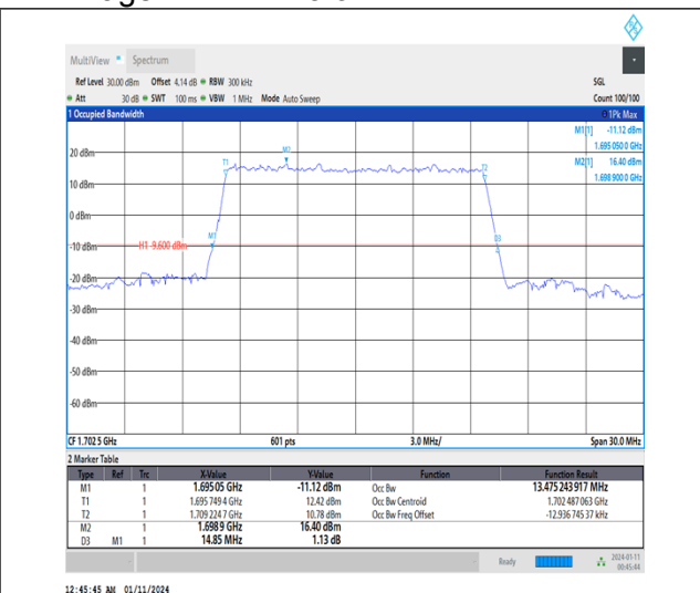
Band70-15MHz-16QAM-133047-75RB#0-PASS
