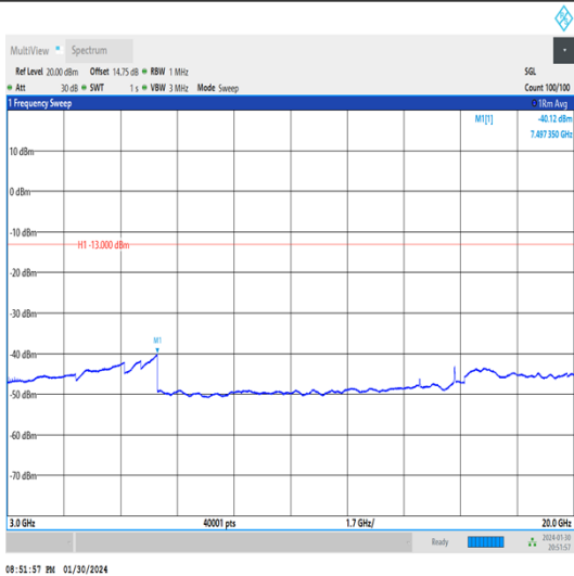
Band70_15MHz_QPSK_133047_1RB#0_3000~20000_30 00~20000
