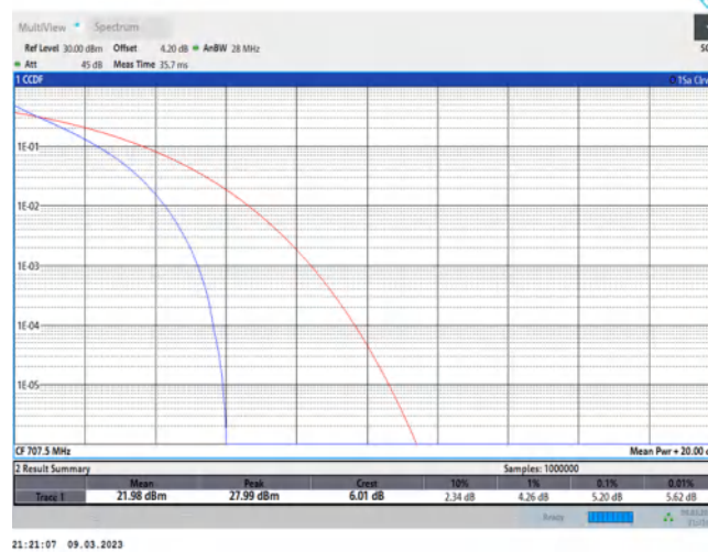
Band12-10MHz-QPSK-23095-50RB#0
