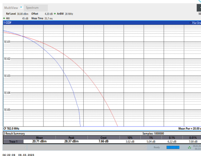
Band13-10MHz-16QAM-23230-50RB#0
