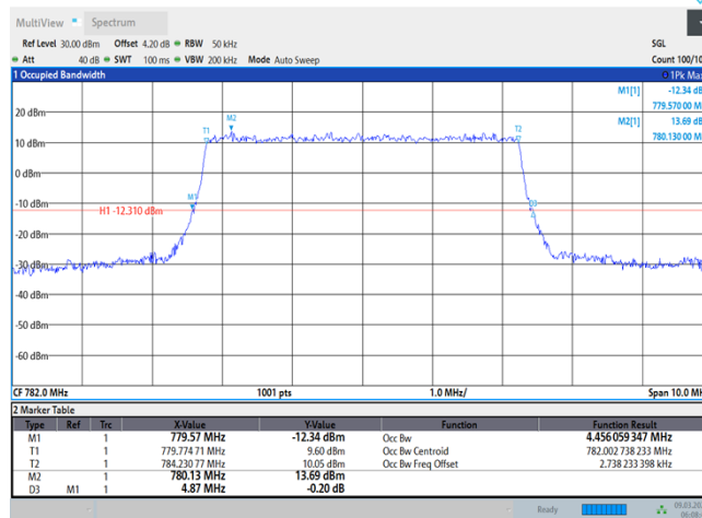
Band13-5MHz-QPSK-23230-25RB#0
