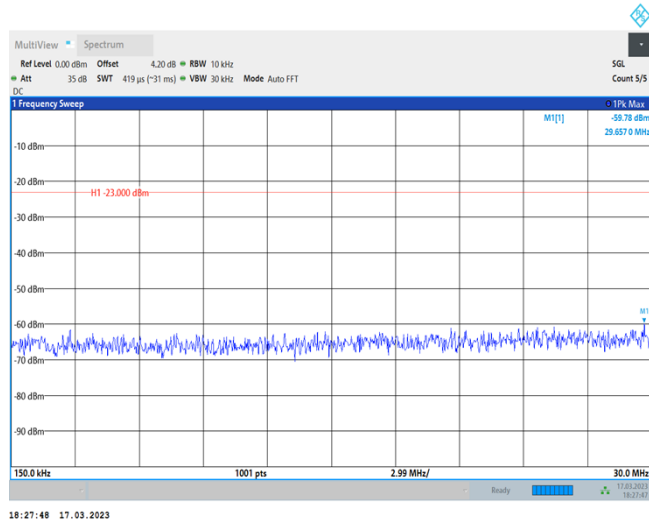
Band17-10MHz-QPSK-23780-1RB#0-Range2:0.15~30MHz
