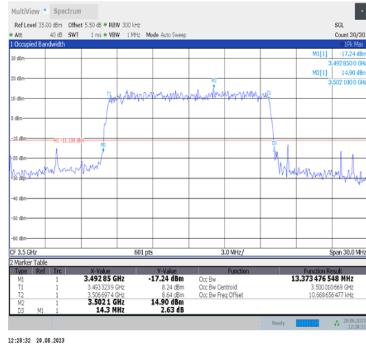
Band42-15MHz-16QAM-42590-75RB#0-PASS
