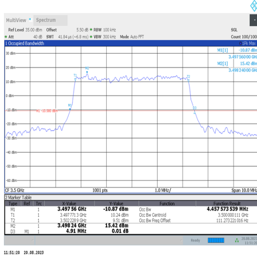
Band42-5MHz-QPSK-42590-25RB#0-PASS
