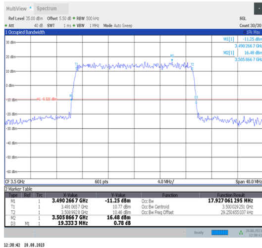
Band42-20MHz-QPSK-42590-100RB#0-PASS
