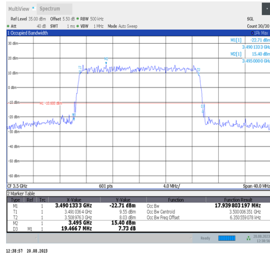
Band42-20MHz-16QAM-42590-100RB#0-PASS
