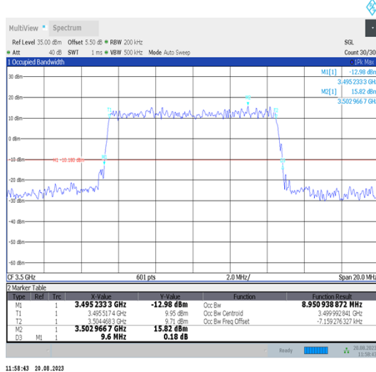
Band42-10MHz-QPSK-42590-50RB#0-PASS
