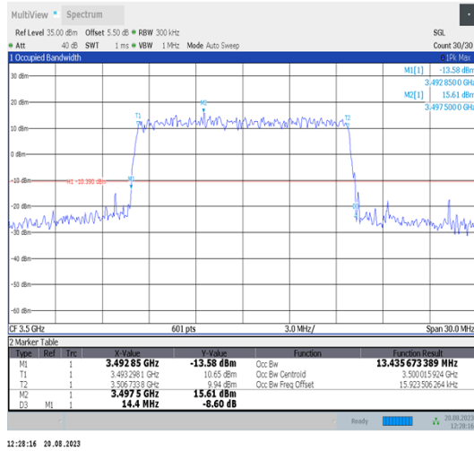
Band42-15MHz-QPSK-42590-75RB#0-PASS
