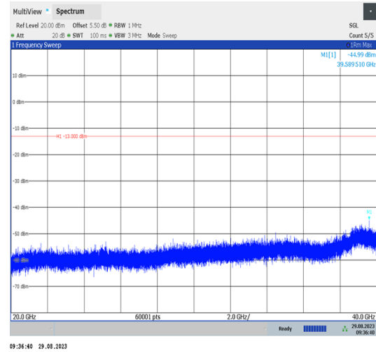
Band42_20MHz_QPSK_42590_1RB#0_20000~40000_20000~40000
