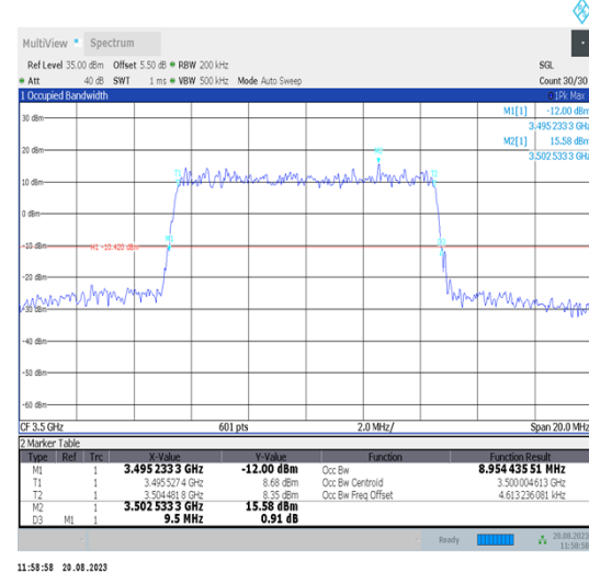
Band42-10MHz-16QAM-42590-50RB#0-PASS
