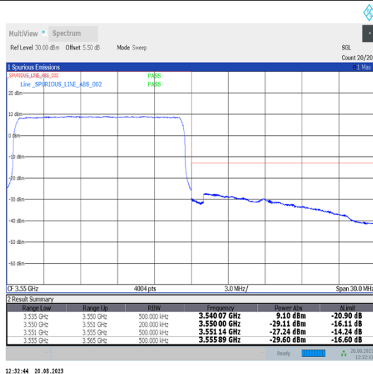
Band22_15MHz_QPSK_43015_75RB#0
