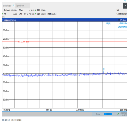
Band42_20MHz_QPSK_42590_1RB#0_0.15~30_0.15~30
