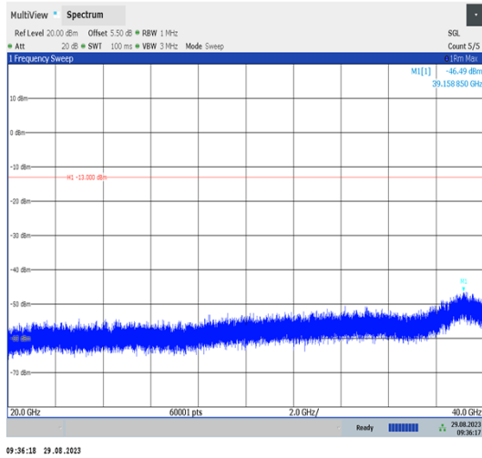
Band42_20MHz_QPSK_42190_1RB#0_20000~40000_20000~40000
