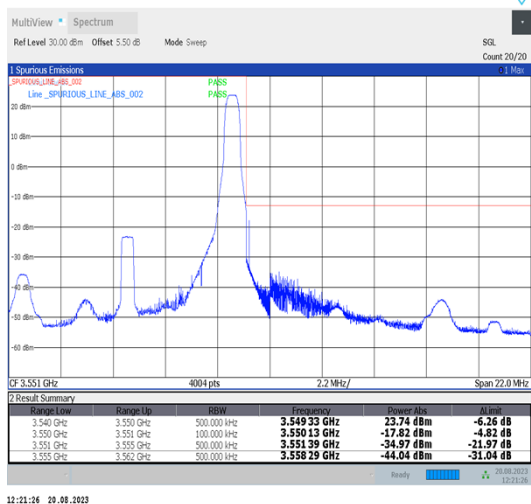
Band22_10MHz_QPSK_43040_1RB#49
