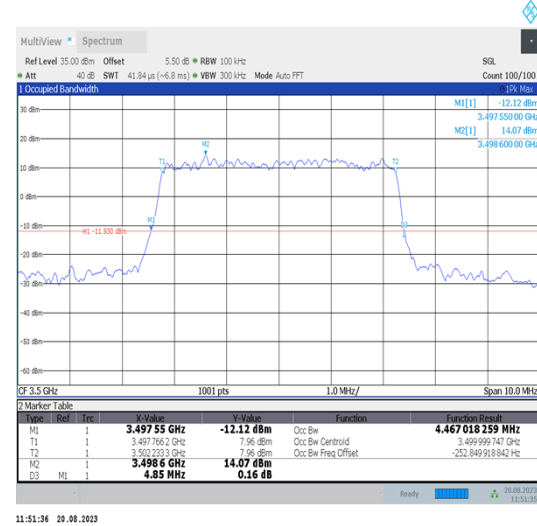
Band42-5MHz-16QAM-42590-25RB#0-PASS
