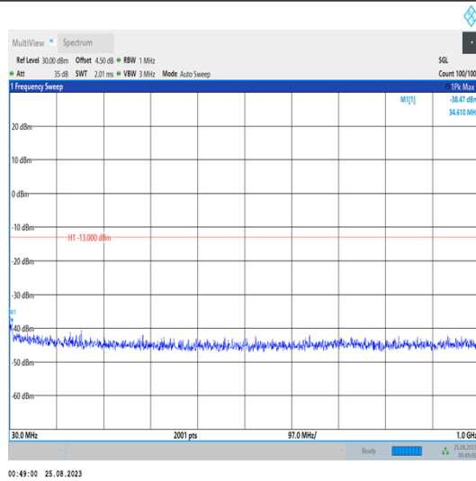
Band42_20MHz_QPSK_42990_1RB#0_30~1000_30~1000
