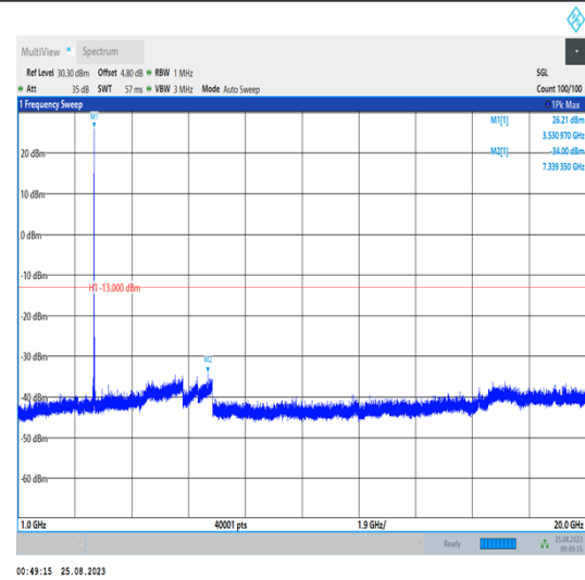
Band42_20MHz_QPSK_42990_1RB#0_1000~20000_1000~20000
