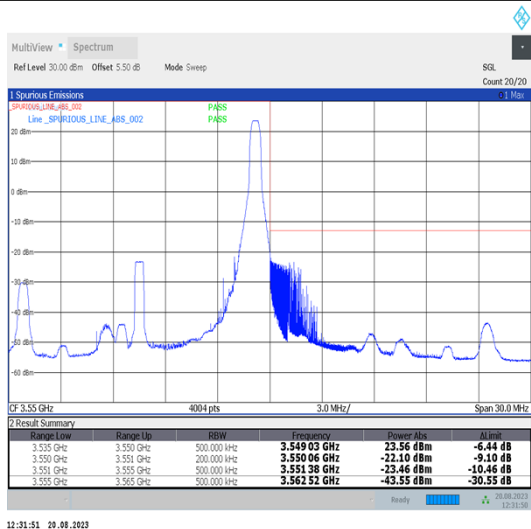
Band22_15MHz_QPSK_43015_1RB#74
