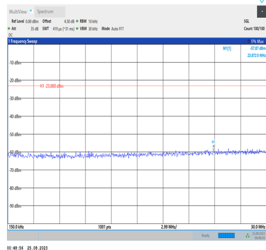
Band42_20MHz_QPSK_42990_1RB#0_0.15~30_0.15~30
