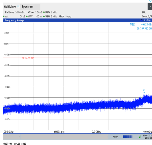
Band42_20MHz_QPSK_42990_1RB#0_20000~40000_20000~40000
