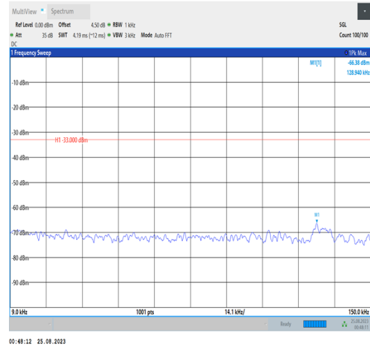
Band42_20MHz_QPSK_42590_1RB#0_0.009~0.15_0.09~0.15
