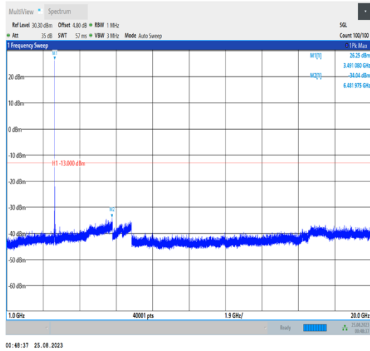
Band42_20MHz_QPSK_42590_1RB#0_1000~20000_1000~20000
