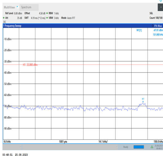
Band42_20MHz_QPSK_42990_1RB#0_0.009~0.15_0.009~0.15
