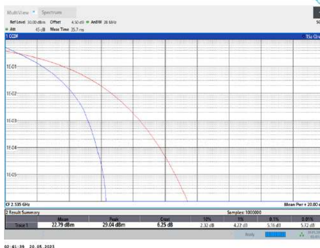
Band7-20MHz-QPSK-21100-100RB#0
