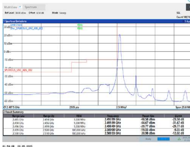
Band7-5MHz-QPSK-20775-25RB#0
