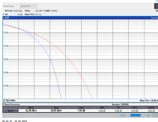
Band13-10MHz-16QAM-23230-50RB#0
