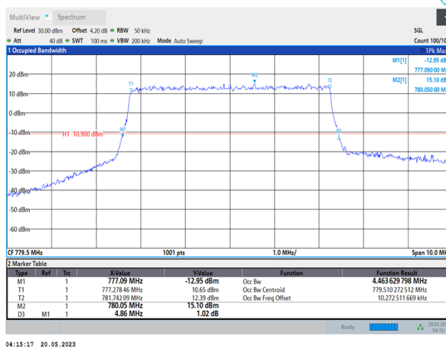
Band13-5MHz-QPSK-23230-25RB#0
