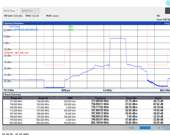
Band14-5MHz-QPSK-23305-25RB#0
