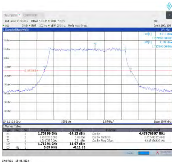
1-N66-PC3-15-5-L-3-DFT-16QAM-Outet_Full-25@0- Ant0-4.48-5.090-<5-PASS
