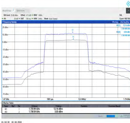
1-N66-PC3-15-40-L-1-DFT-256QAM-Outer_Full-216 @0-Ant0-9.13-100%-0.00-9.13-PASS-≤13
