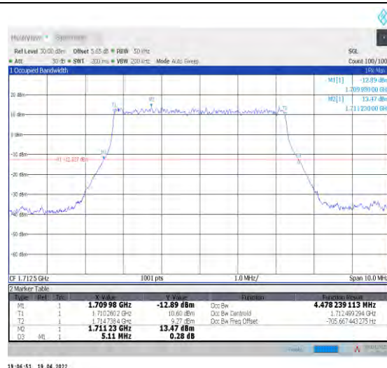
1-N66-PC3-15-5-L-2-DFT-PI2BPSK-Outet_Full-25@ 0-Ant0-4.478-5.110-<5-PASS
