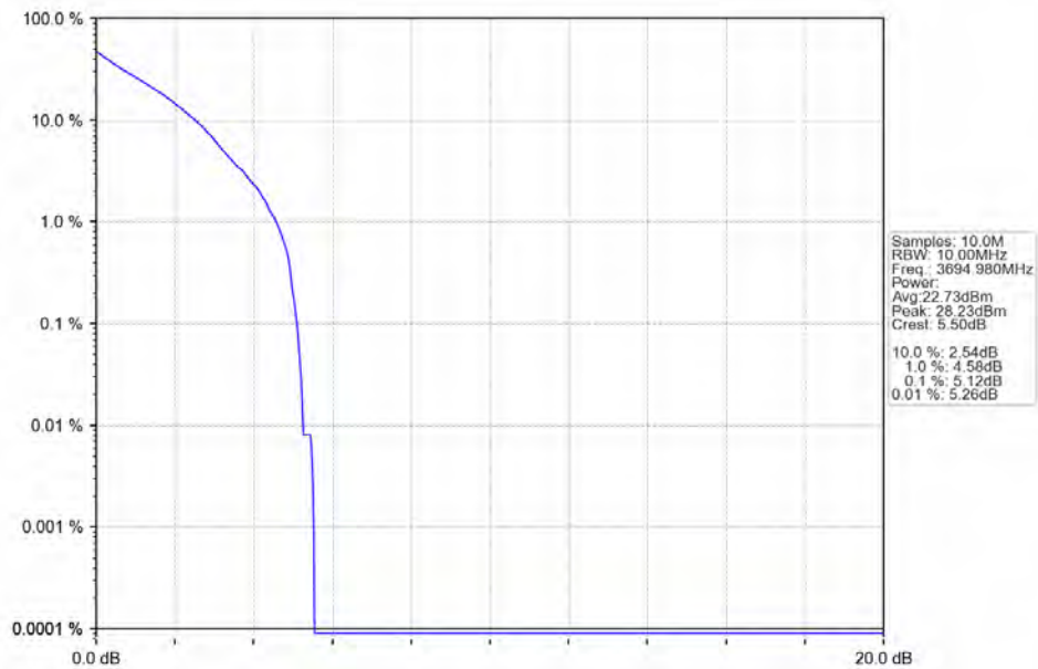
n48_30kHz_SISO_NTNV_10MHz_DFT-s-OFDM_QPSK_3694.98MHz_Outer_Full_Ant1
