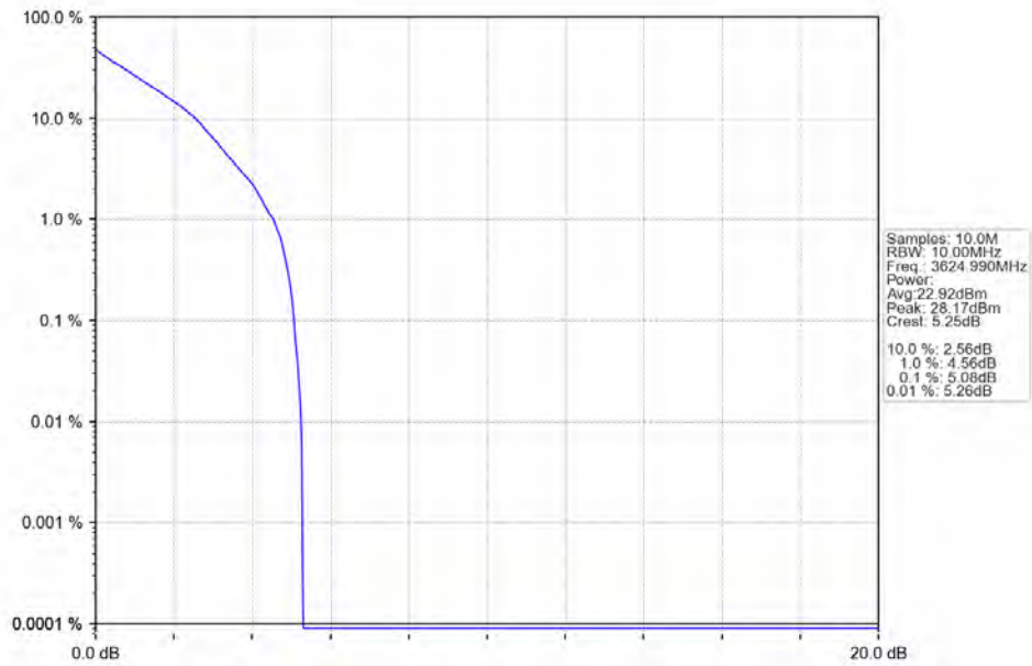
n48_30kHz_SISO_NTNV_10MHz_DFT-s-OFDM_QPSK_3624.99MHz_Outer_Full_Ant1
