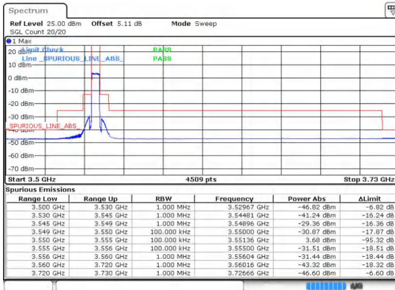
Band48-5MHz-QPSK-55265-25RB#0
