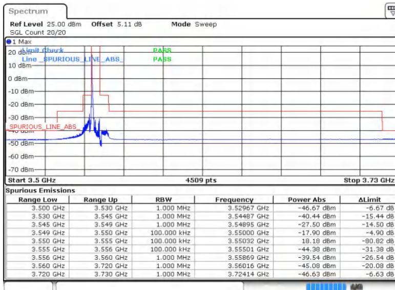
Band48-5MHz-QPSK-55265-1RB#0
