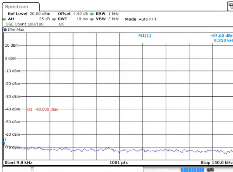
Band48-20MHz-QPSK-55340-1RB#0-Range1:0.009~0.15MHz
