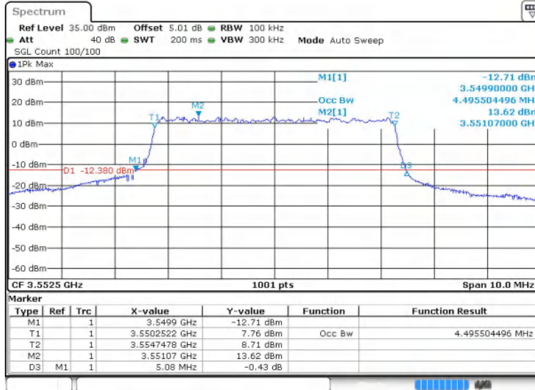
Band48-5MHz-QPSK-55265-25RB#0
