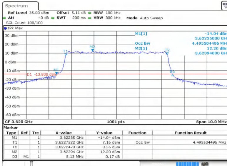
Band48-5MHz-QPSK-55990-25RB#0
