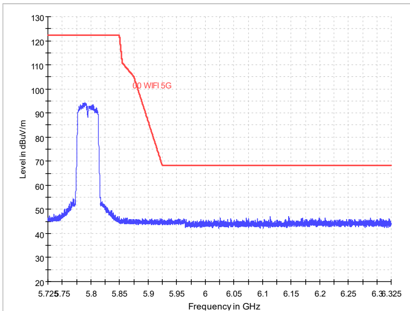
Radiated Emission Band Edge Channel No.:159 Test Mode: 802.11ac Polarization: H
