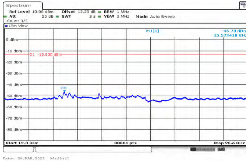
Band2-1.4MHz-16QAM-18900-1-0-Low-30-1000--33.19-PASS
