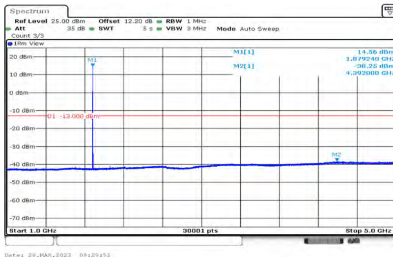
Band2-1.4MHz-16QAM-18900-1-0-Low-1000-5000--38.25-PASS
