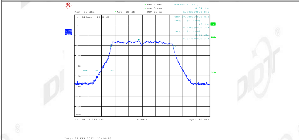
11N40MIMO Ant2 5795
