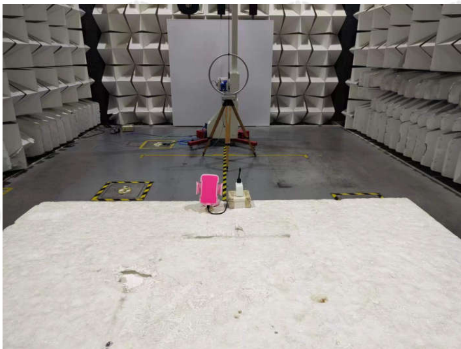
Radiated Spurious Emissions Test Setup-1 (9kHz~30MHz)
