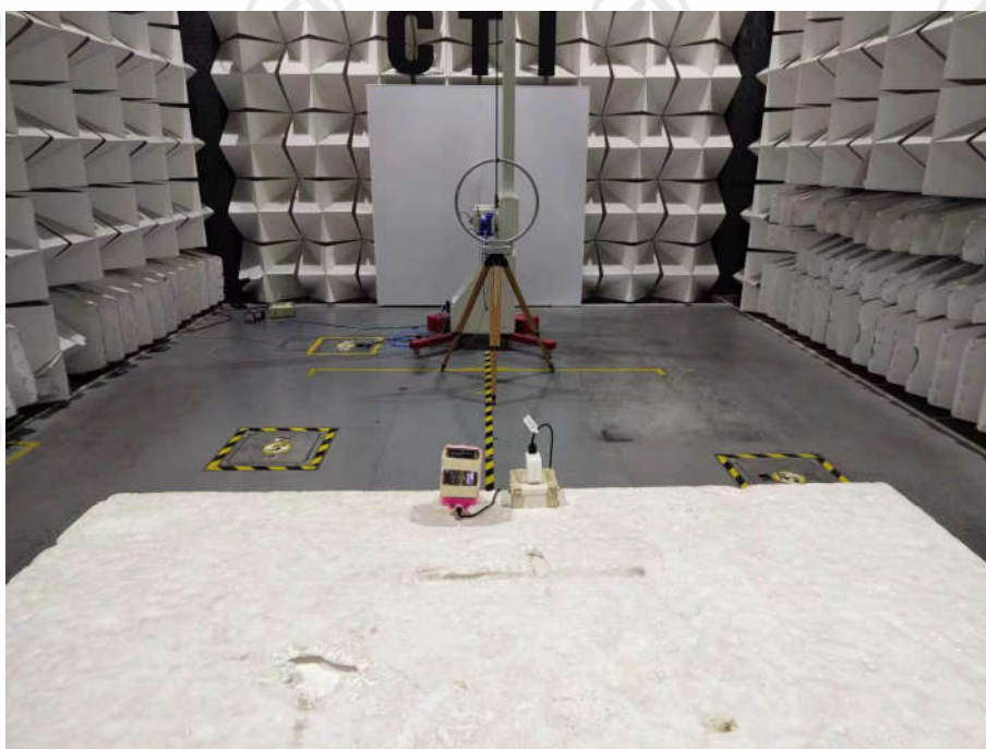
Radiated Spurious Emissions Test Setup-2 (9kHz~30MHz)
