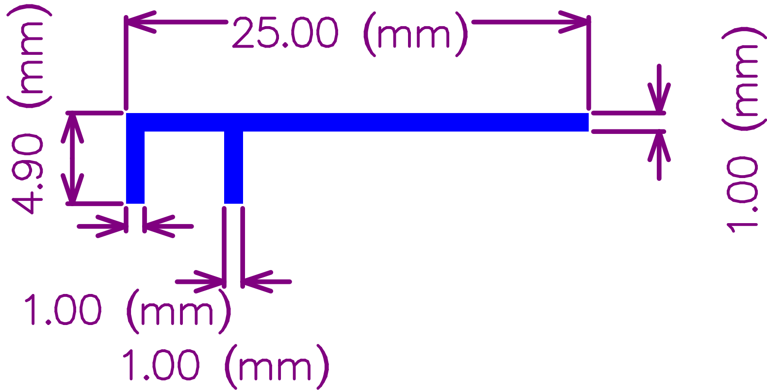
Antenna Dimension Drawing
